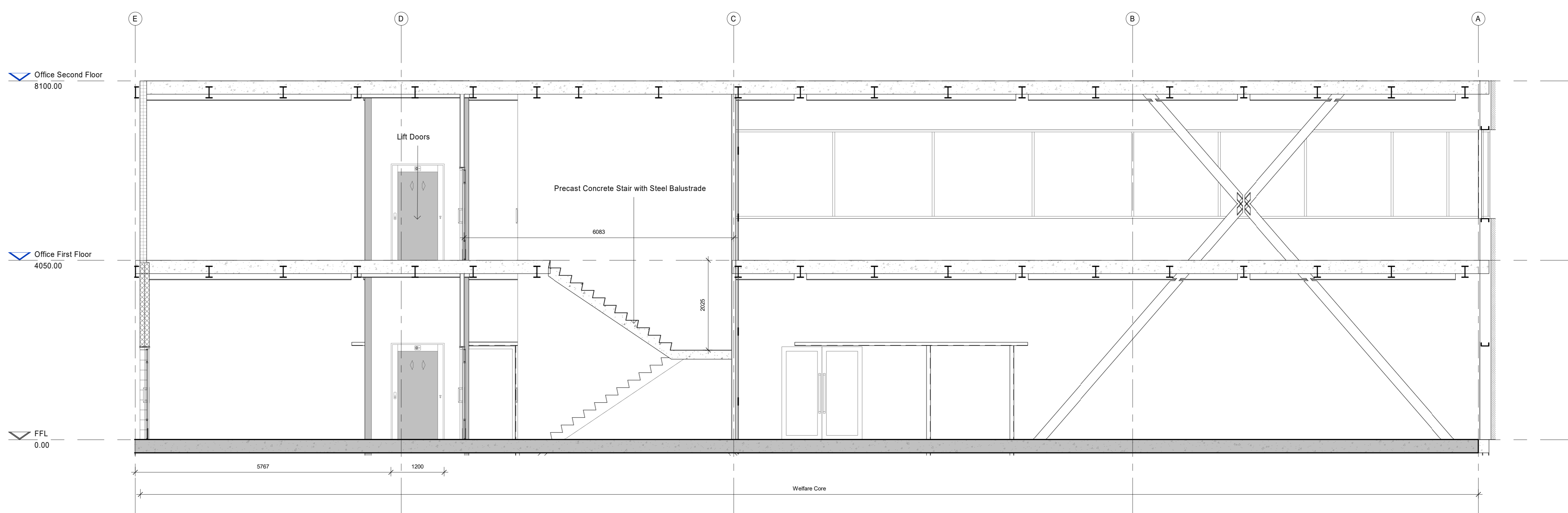
3 Welfare Area Section 2 1 : 50
