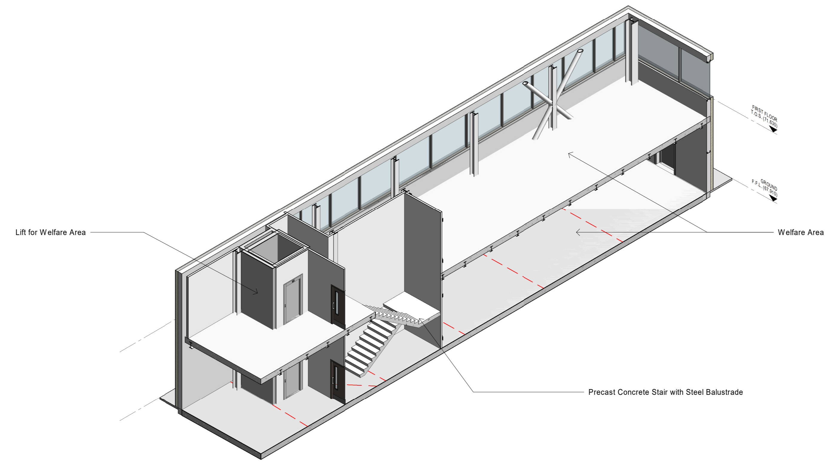
4 Welfare Area 3D
