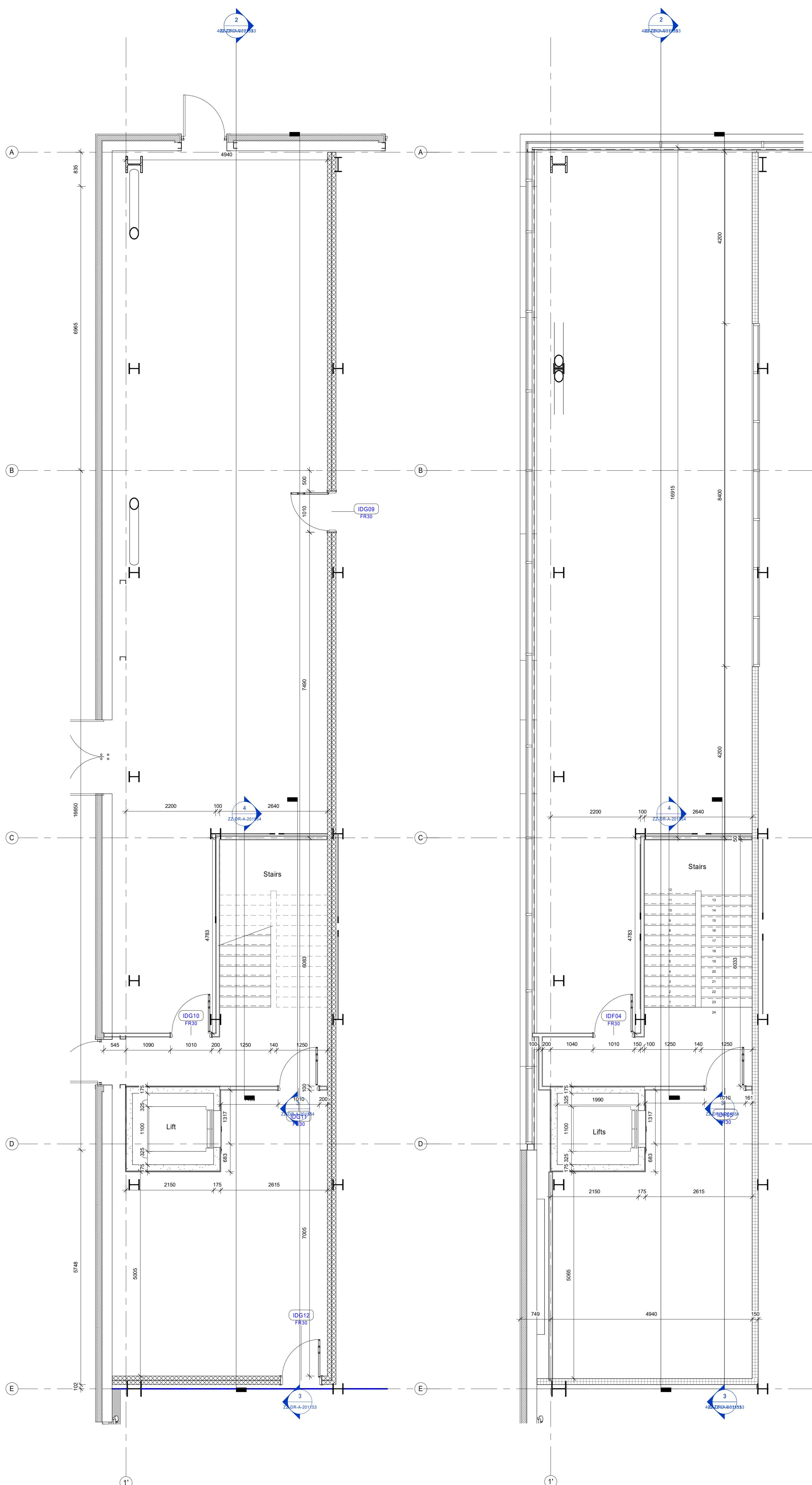
1 Welfare Area Plan 1 : 50
