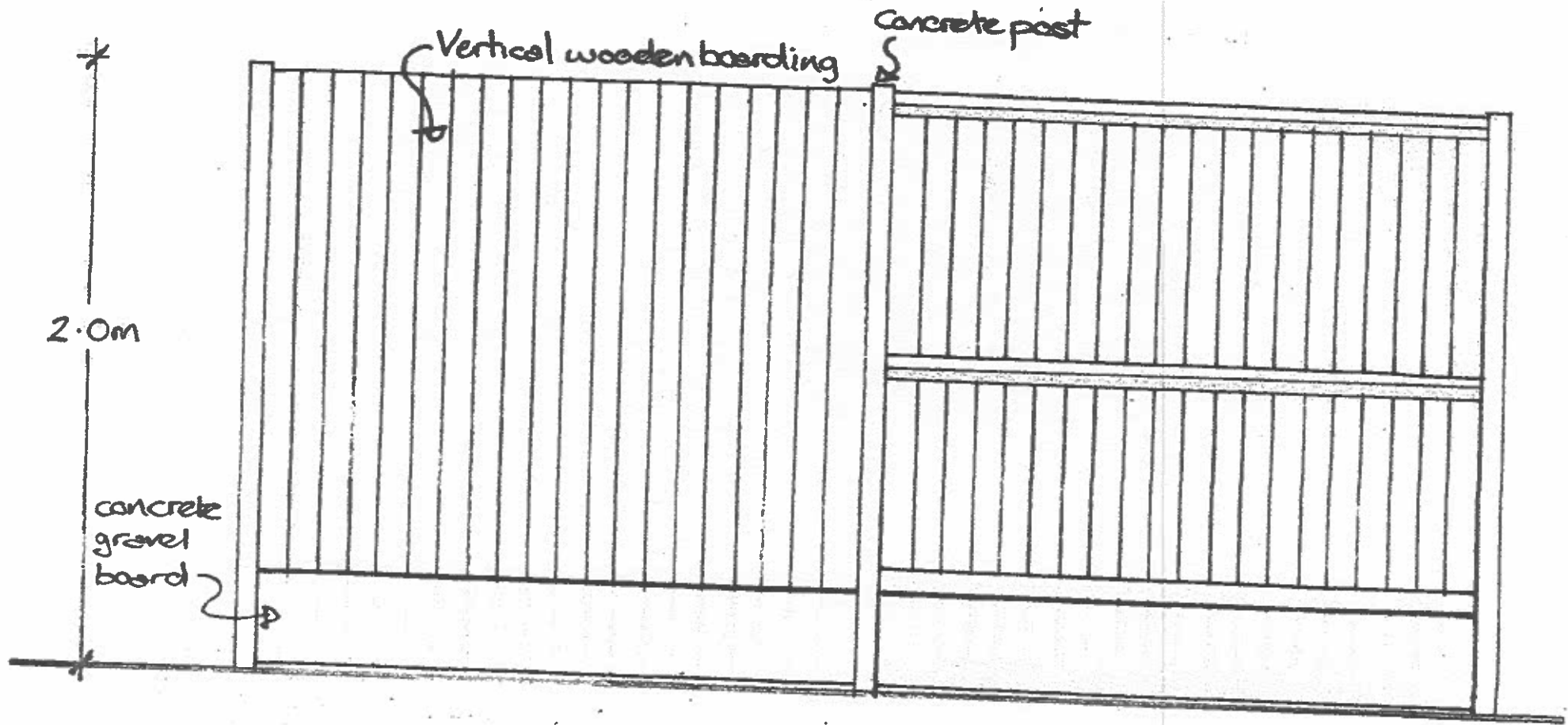
FRONT ELEVATION
