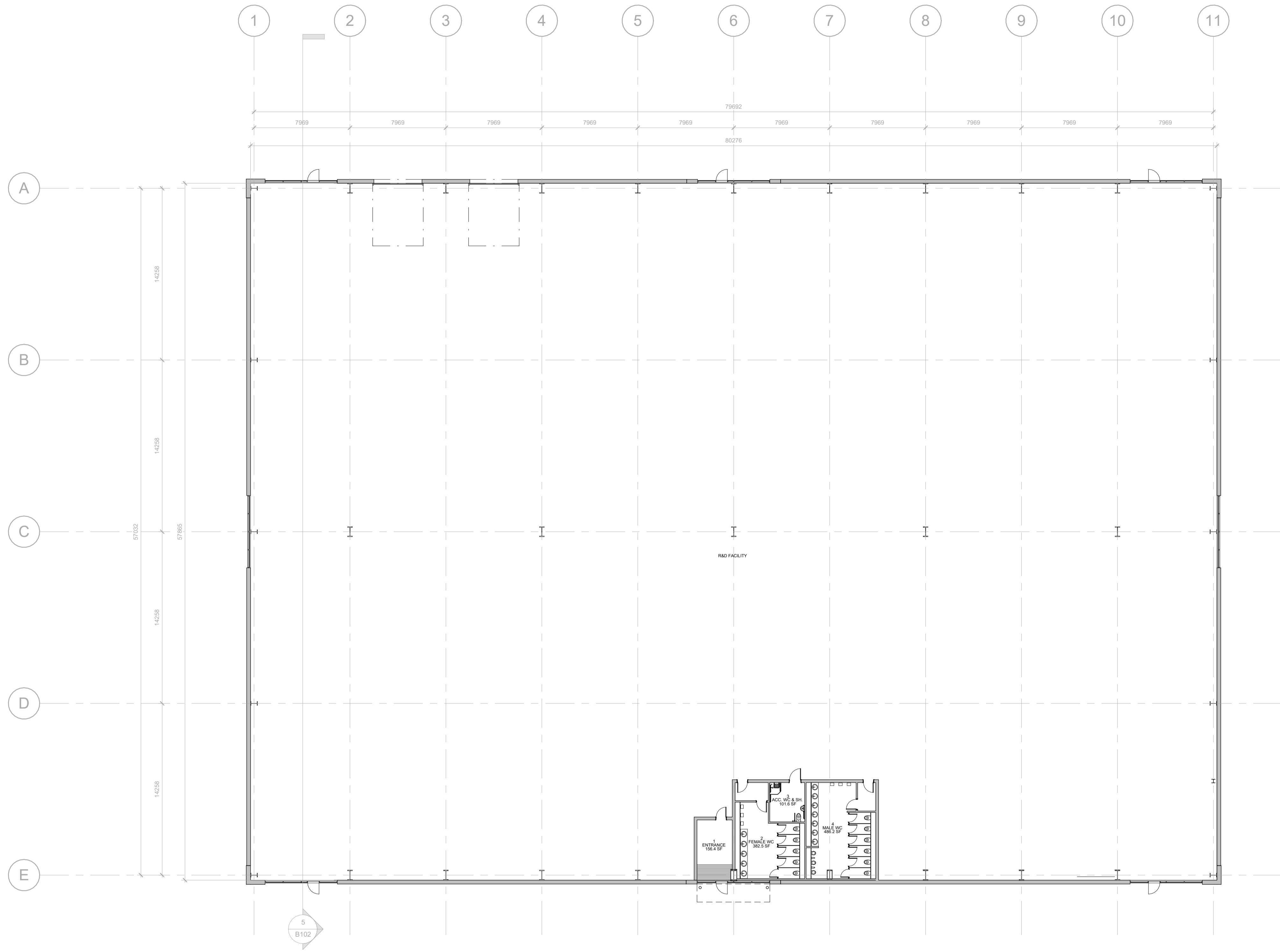
Ground Floor 1 : 200
