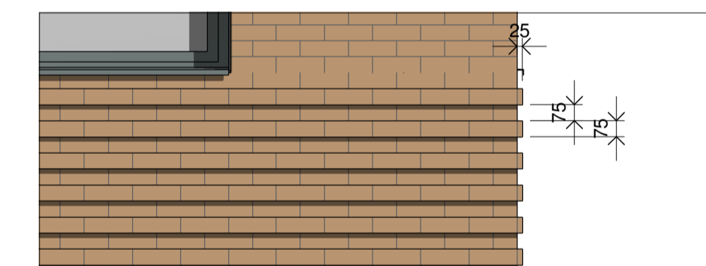
3 Brick projecting stretcher courses 1 : 25
