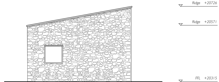
North elevation
