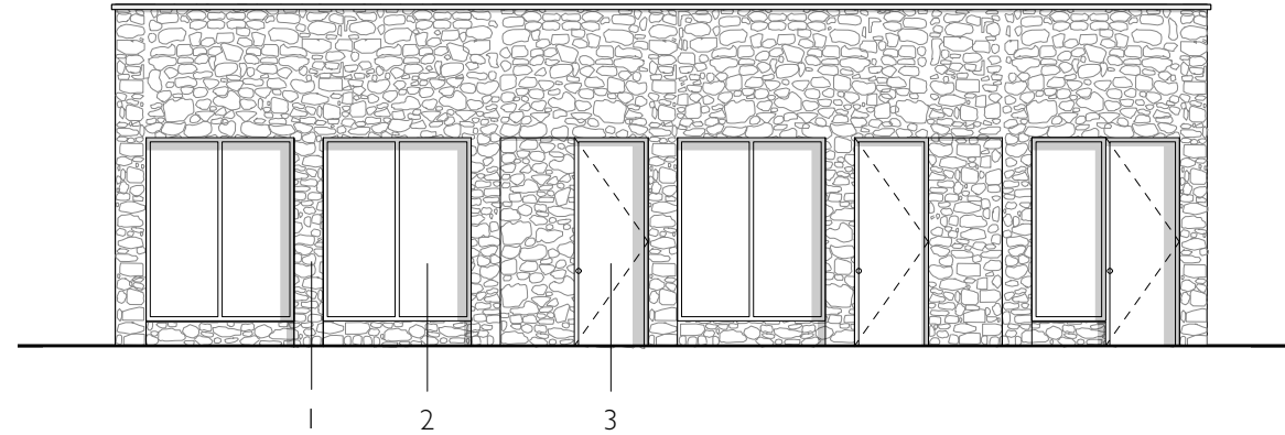
West elevation
