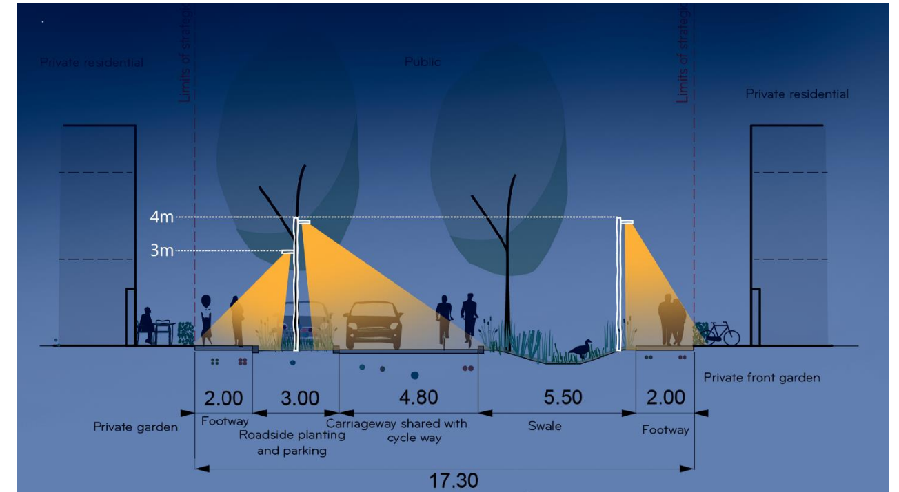
Figure 6.12–Lighting strategy for a typical secondary street with swale
