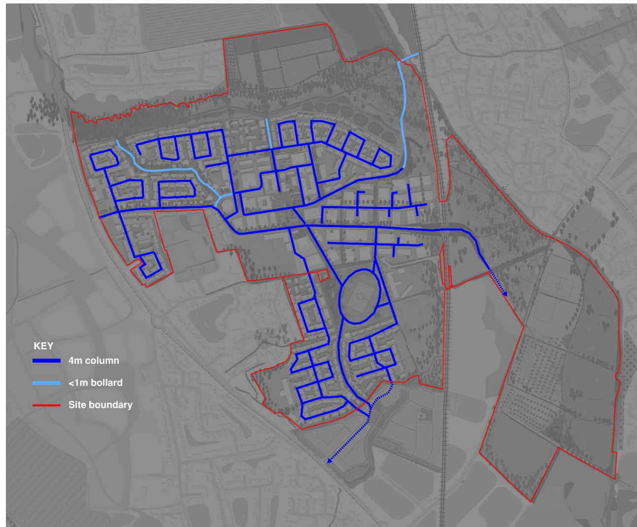
Figure 6.4 – Illustrative light source mounting heights
