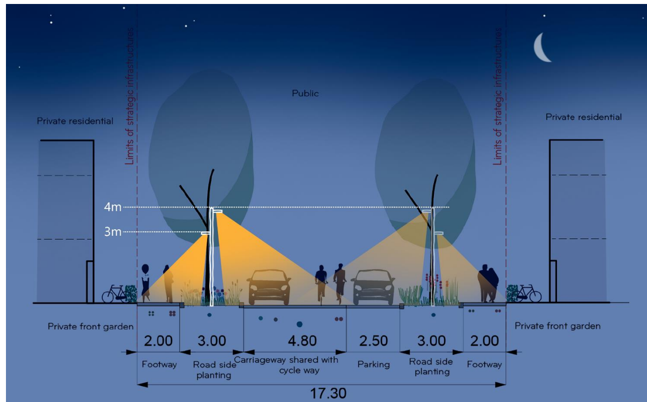
Figure 6.11 – Lighting strategy for a typical secondary street
