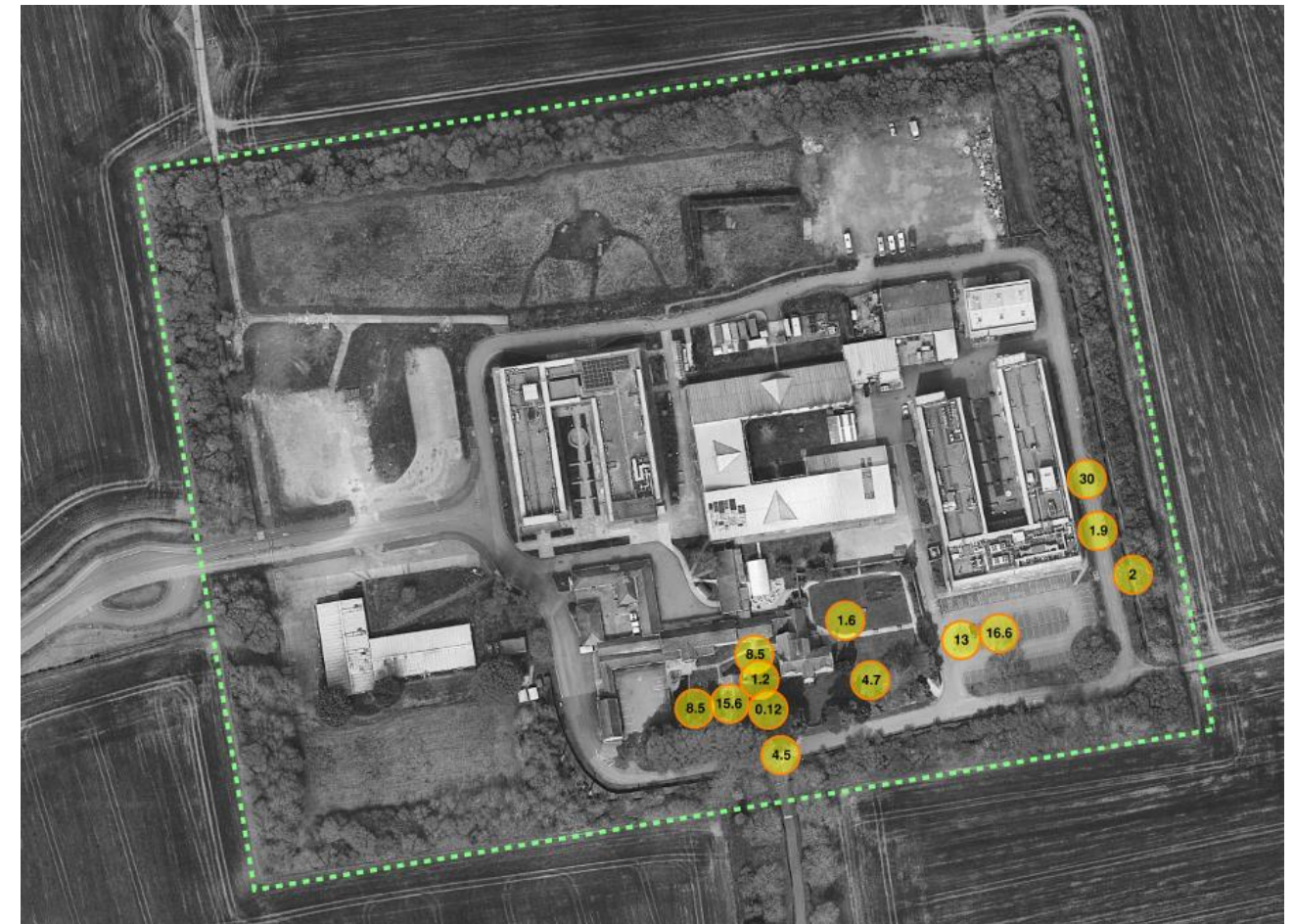
Figure 2.24– Existing Illumination levels within Begbroke science park noted in values of Lux.
