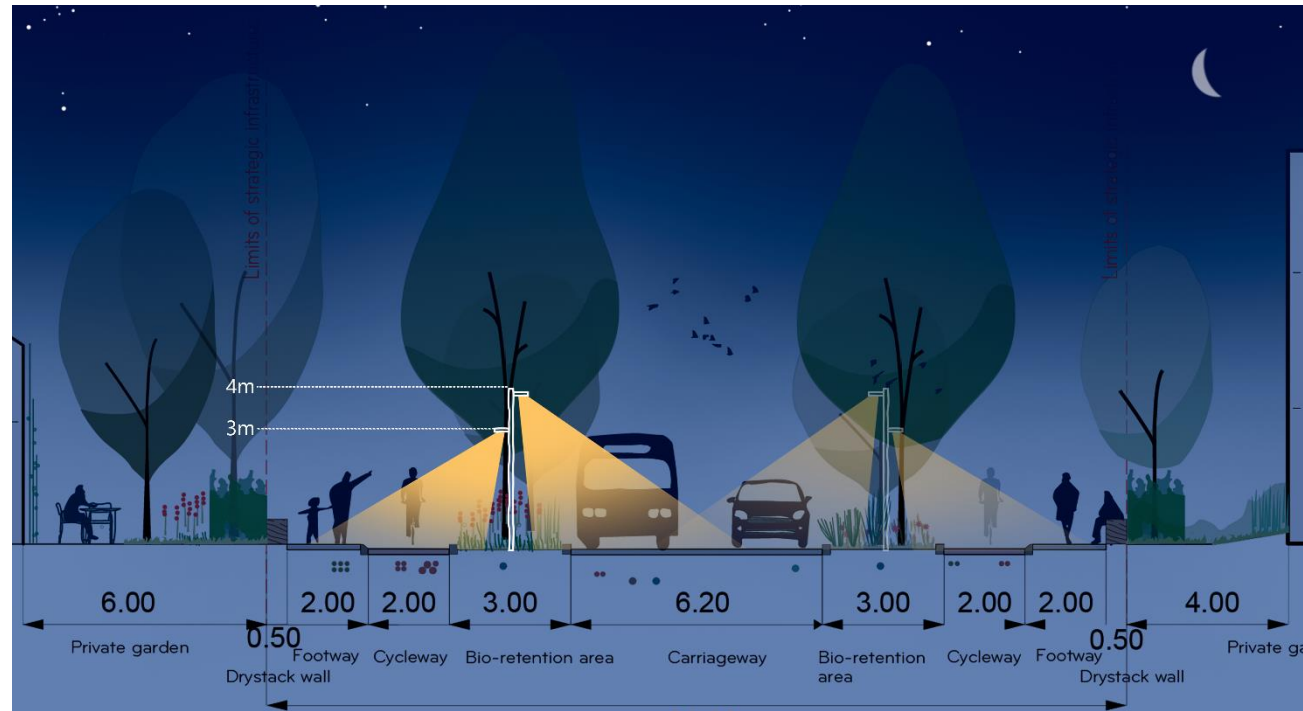
Figure 6.10 – Lighting strategy for Begbroke Hill Road
