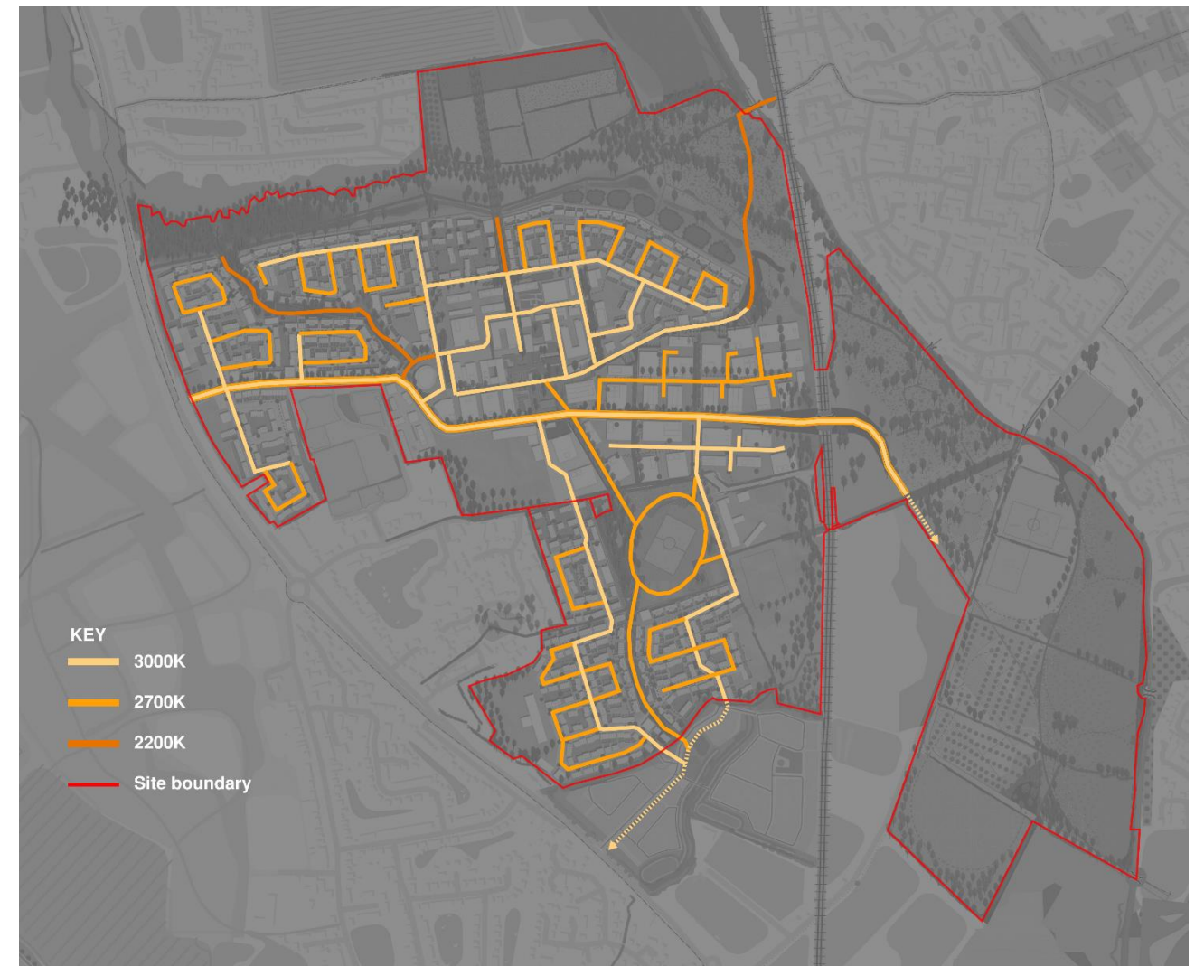
Figure 6.3. – Illustrative lighting colour temperature strategy
