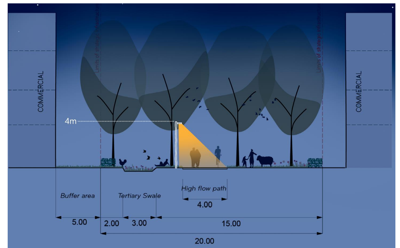
Figure 6.13 –Lighting strategy for a typical high flow shared surface path
