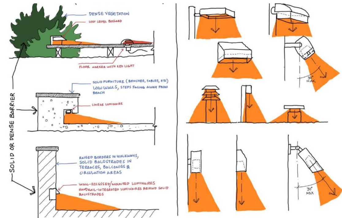
Figure 6.5 – Integrated and external shielding methods
