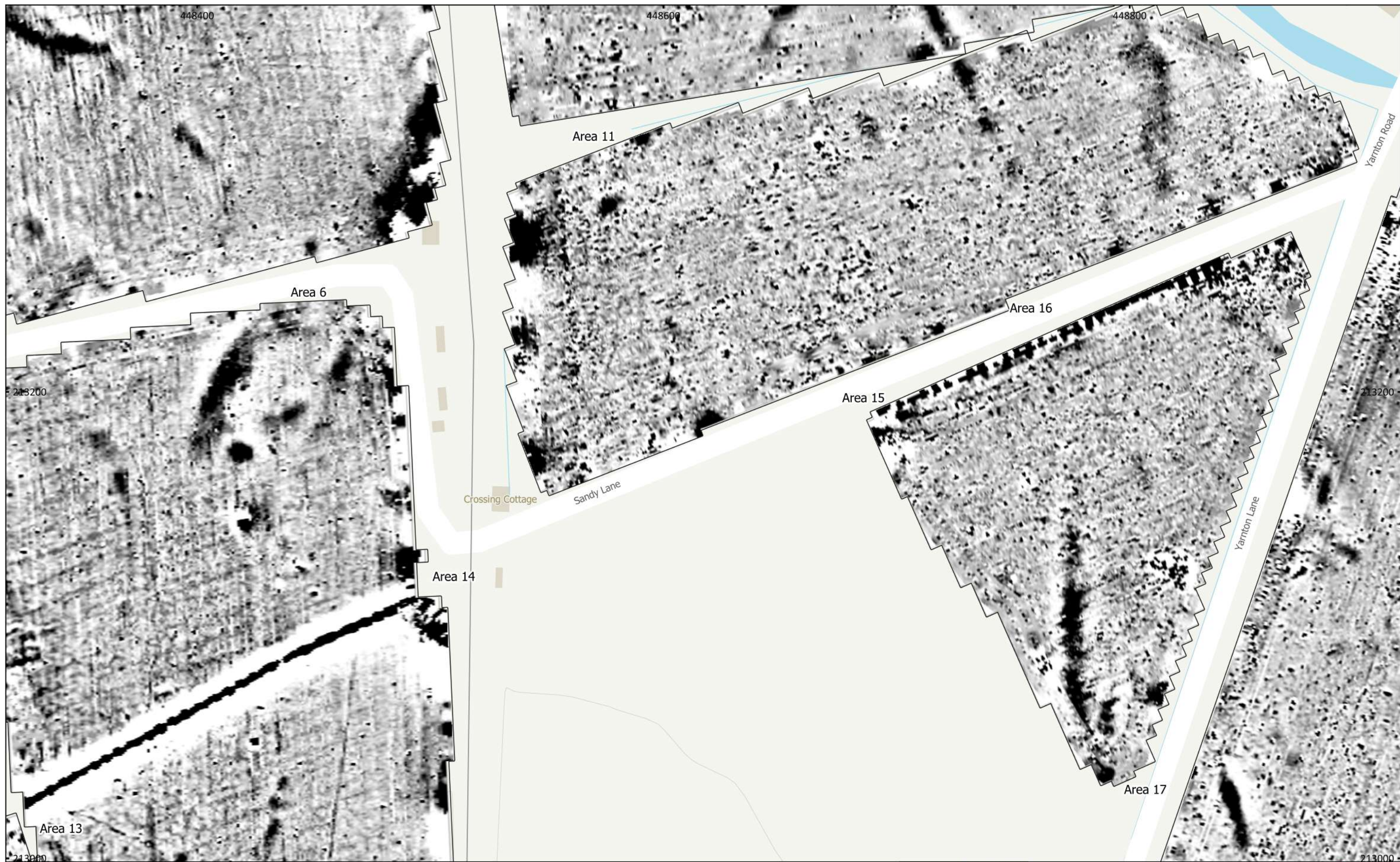
MSSP1306 - Begbroke, Oxfordshire Figure 44 - Magnetic Gradient (Areas 6, 11, 14, 15, 16 & 17) 1:1,500 @ A3 Copyright Magnitude Surveys Ltd 2022 Contains Ordnance Survey data © Crown Copyright and database right 2022
