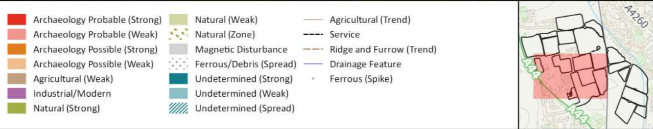
MSSP1306 - Begbroke, Oxfordshire Figure 18 - Magnetic Interpretation Over Historical Maps and Satellite Imagery (Overview) (Central Area) 1:3,000 @ A3 Copyright Magnitude Surveys Ltd 2022 Contains historical mapping © CLS Data 2022: Ordnance Survey, 6" 2nd edition c. 1882-1913 Contains satellite imagery © 2022 Bing Satellite
