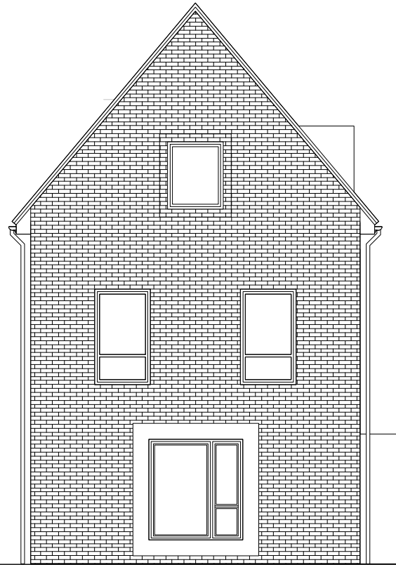
SIDE ELEVATION
