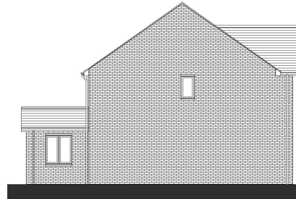
SIDE ELEVATION
