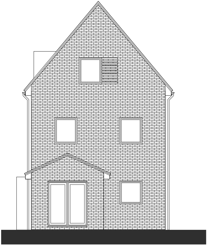
SIDE ELEVATION
