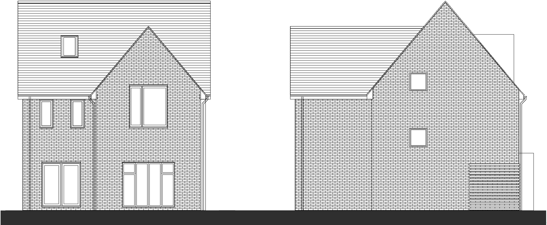
REAR ELEVATION
