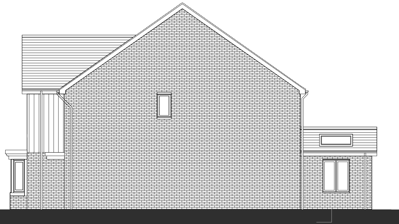
SIDE ELEVATION
