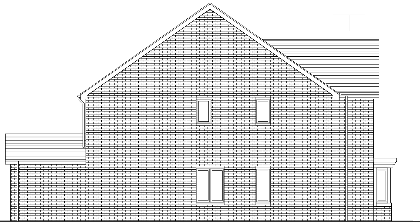
SIDE ELEVATION
