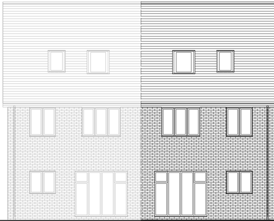
REAR ELEVATION
