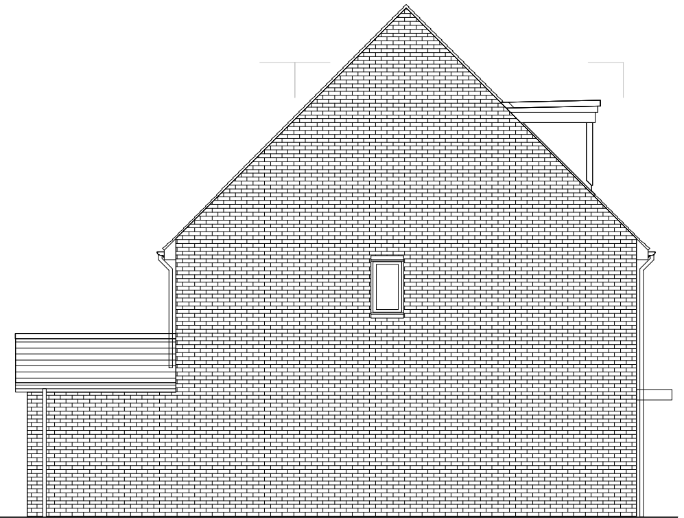
SIDE ELEVATION
