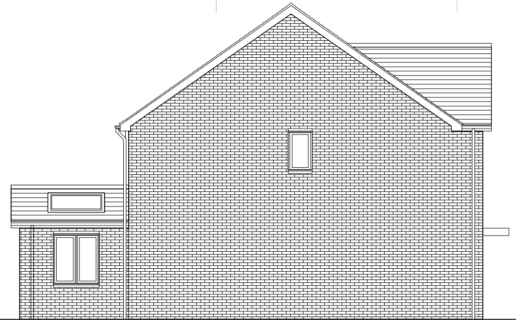
SIDE ELEVATION
