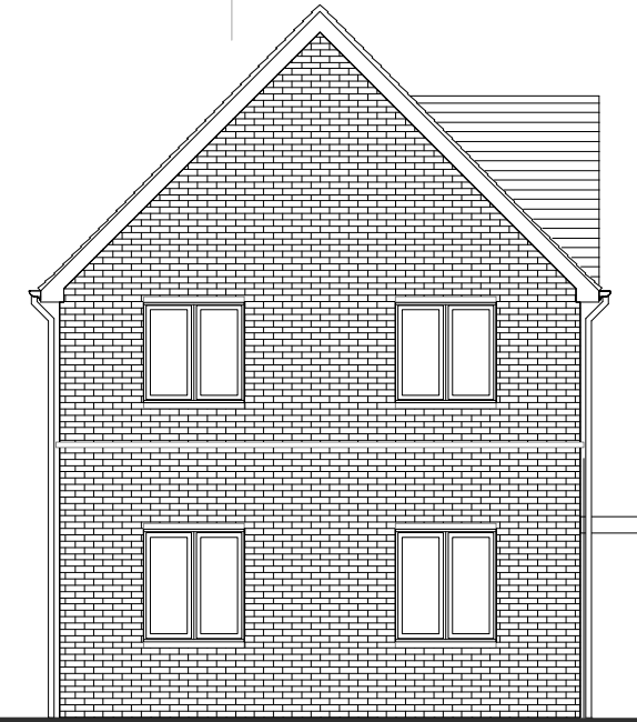
SIDE ELEVATION
