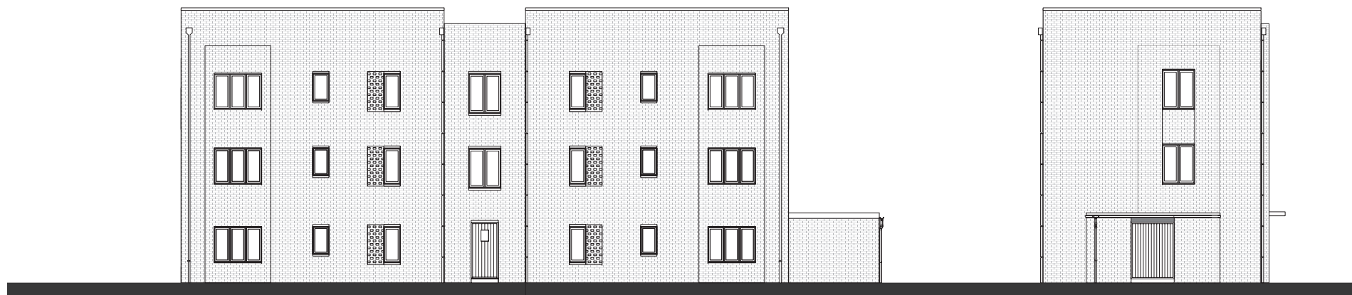
REAR ELEVATION
