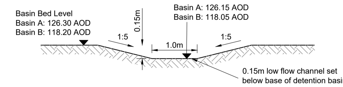
TYPICAL LOW FLOW CHANNEL (Refer to drawing DR-C-5602 & 5603 for location and layout) SCALE 1:50
