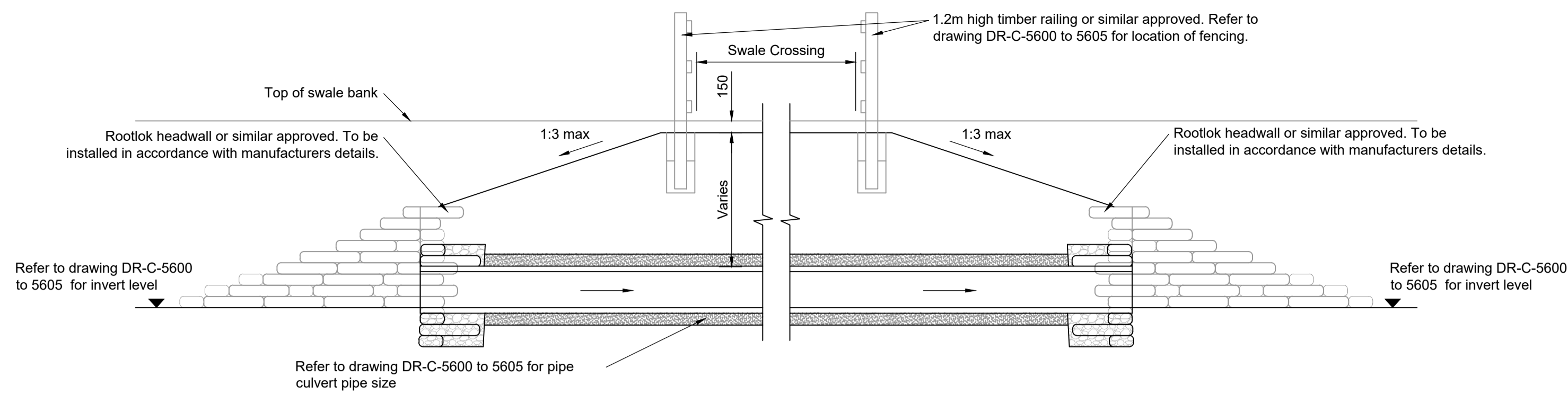
TYPICAL SWALE CULVERT SECTION (PIPE Ø >300mm) Scale 1:50
