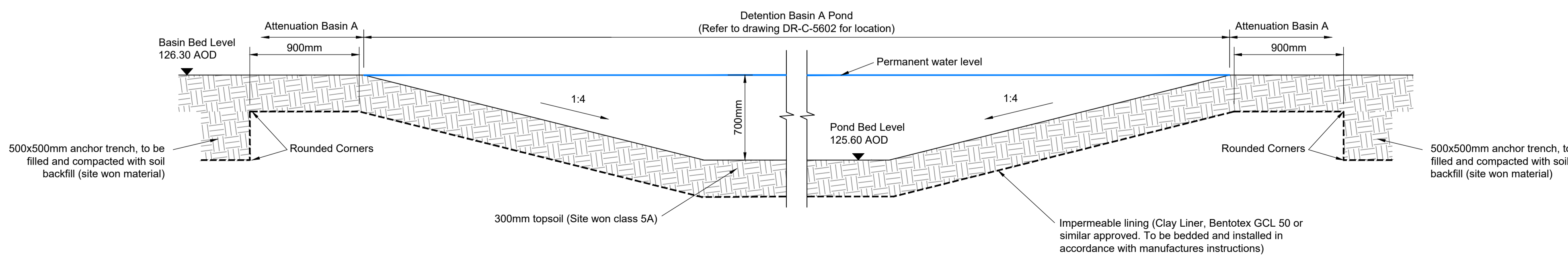
POND DETAIL (Attenuation basin a, pond not provided in attenuation basin B) SCALE 1:25
