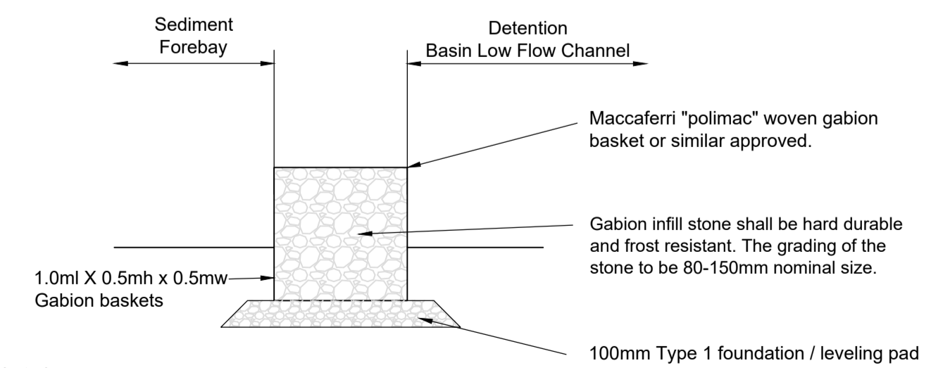
TYPICAL GABION BASKET BERM SECTION Scale 1:20
