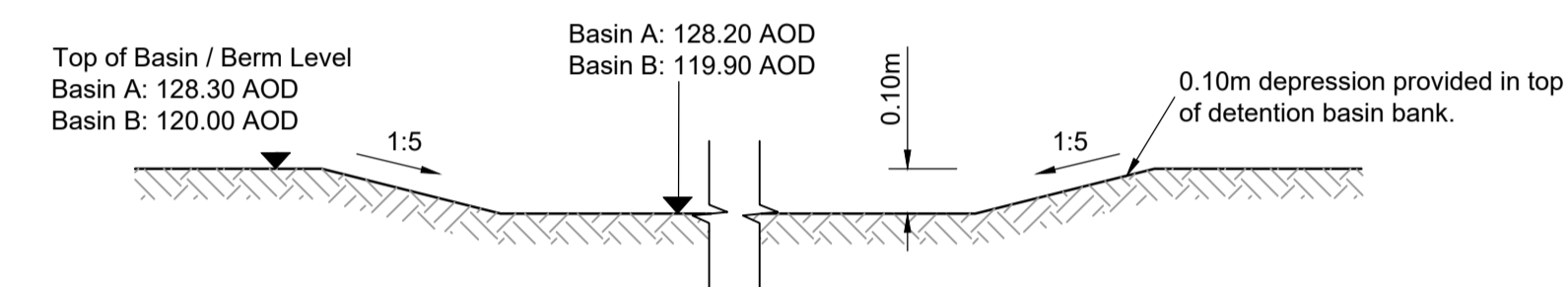
DETENTION BASIN EMERGENCY OVERFLOW (Refer to drawing DR-C-5602 & 5603 for location and layout) SCALE 1:50
