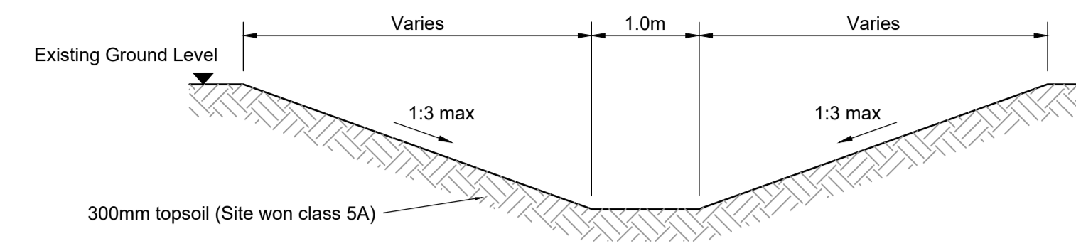
TYPICAL SWALE SECTION (Refer to drawing DR-C-5260 for site specific swale sections and drawing DR-C-5600 to 5603 for location and layout) SCALE 1:50
