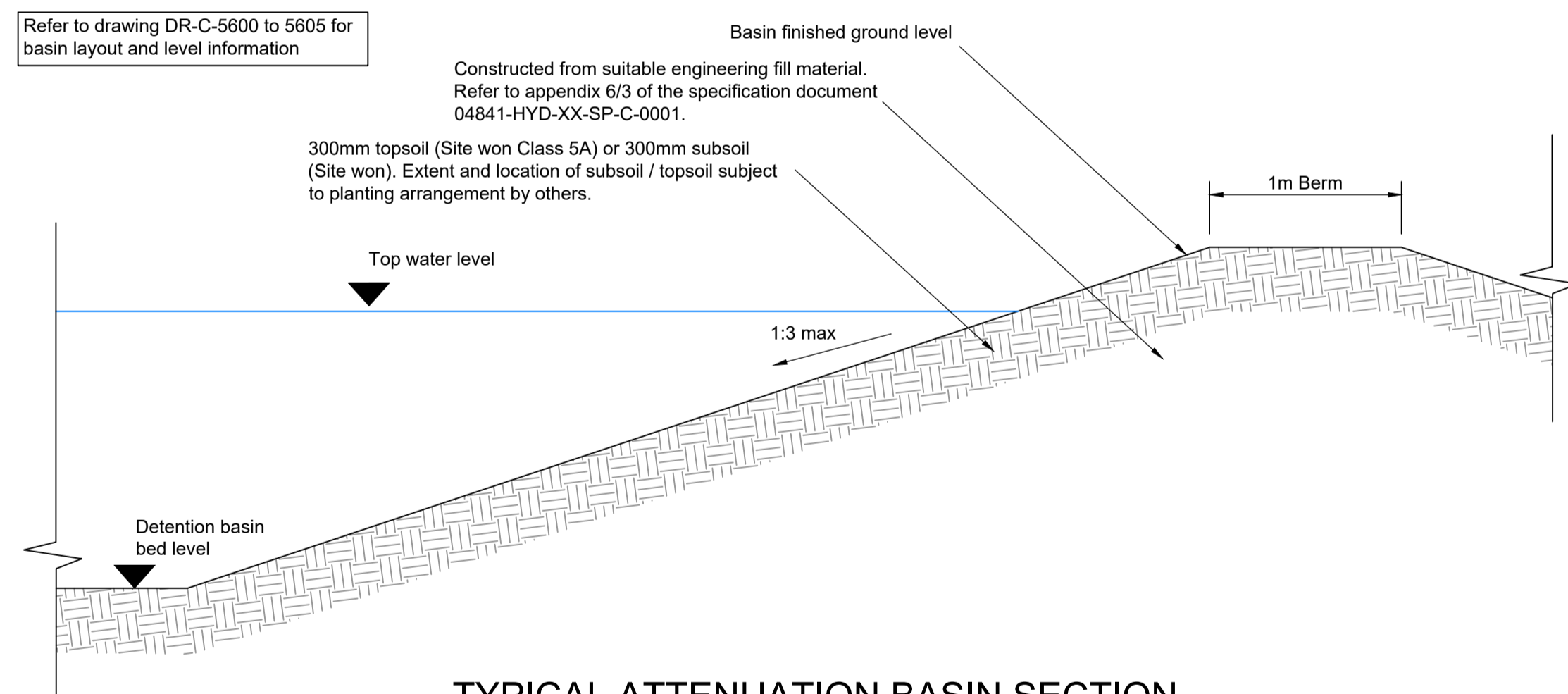
TYPICAL ATTENUATION BASIN SECTION (Attenuation Basin A & B Side Slopes) SCALE 1:25
