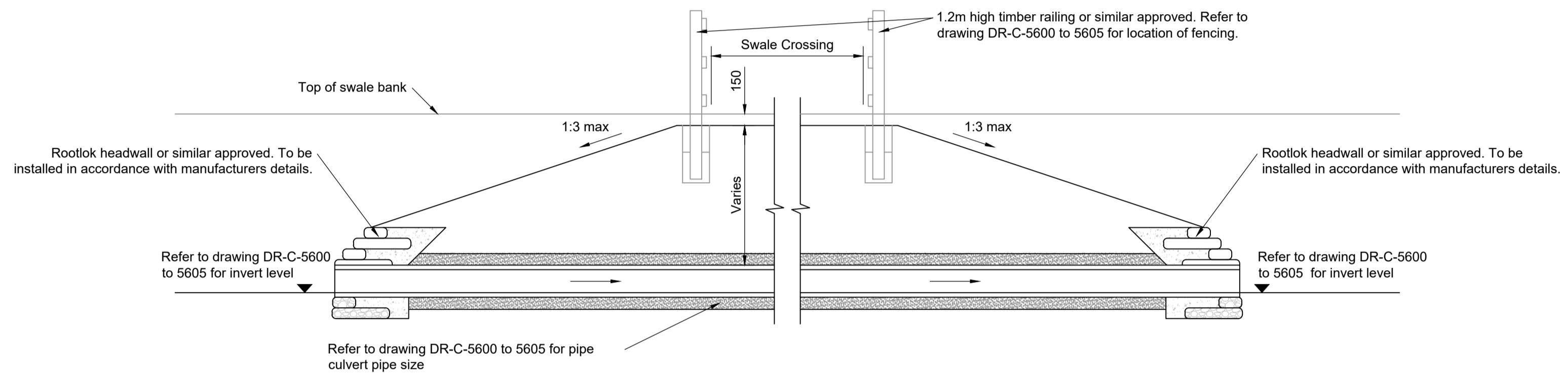
TYPICAL CULVERT SECTION (PIPE Ø ≤300mm) Scale 1:50
