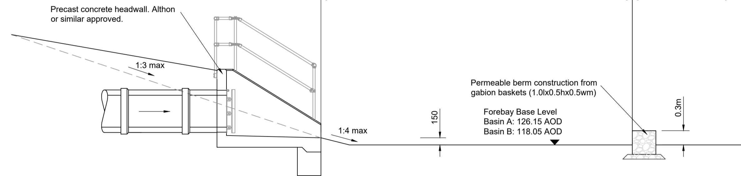
TYPICAL SEDIMENT FOREBAY SECTION (Detention Basin A & B Inlets) Scale 1:50
