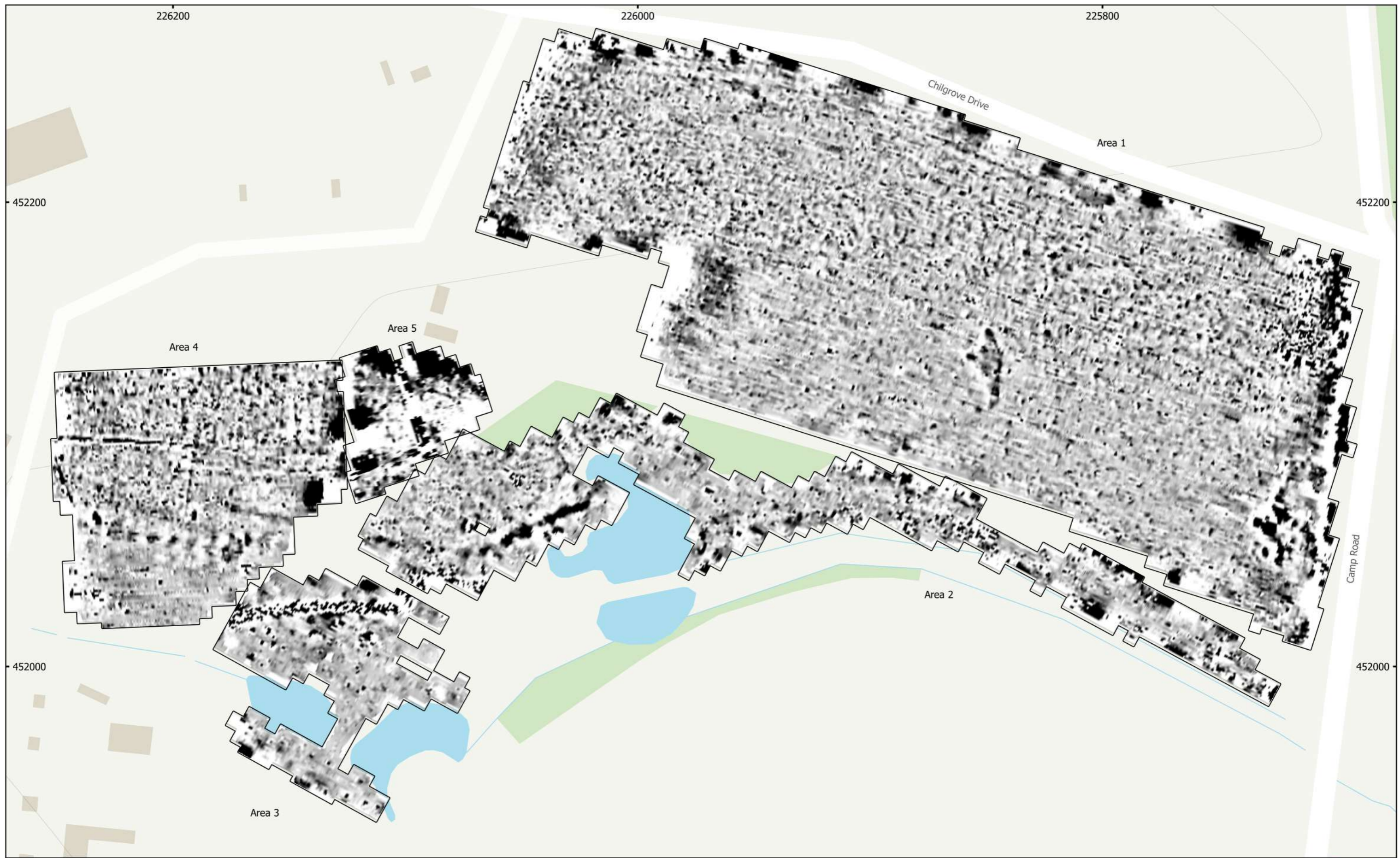
MSSP1040 - Camp Road, Heyford Park Figure 4 - Magnetic Gradient 1:1,500 @ A3 Copyright Magnitude Surveys Ltd 2021 Contains Ordnance Survey data © Crown Copyright and database right 2021
