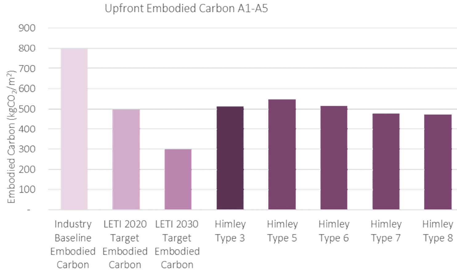
Figure 7 - Embodied (upfront) carbon emissions for the proposed development compared to a number of difference benchmarks
