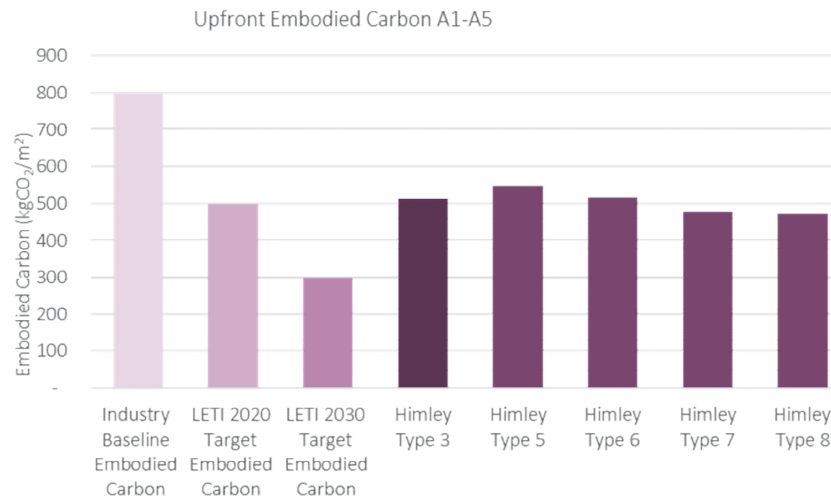
Figure 4 - Upfront carbon for Himley Village house types compared with a number of benchmarks
