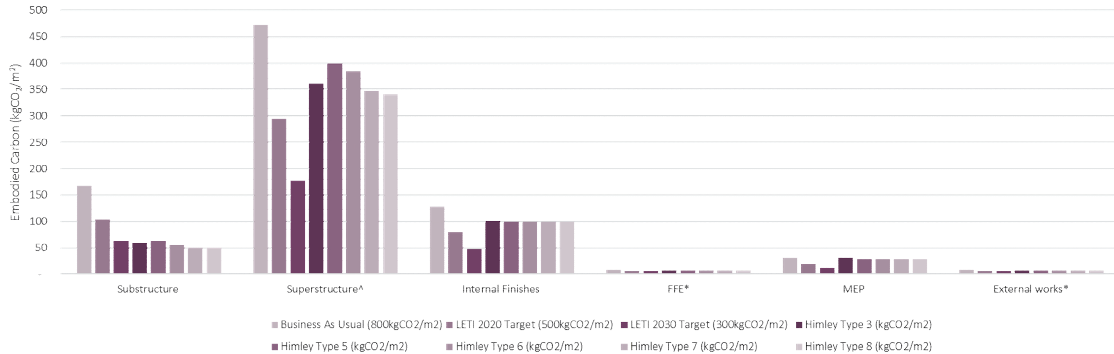
Figure 6 - Embodied carbon breakdown by building element
