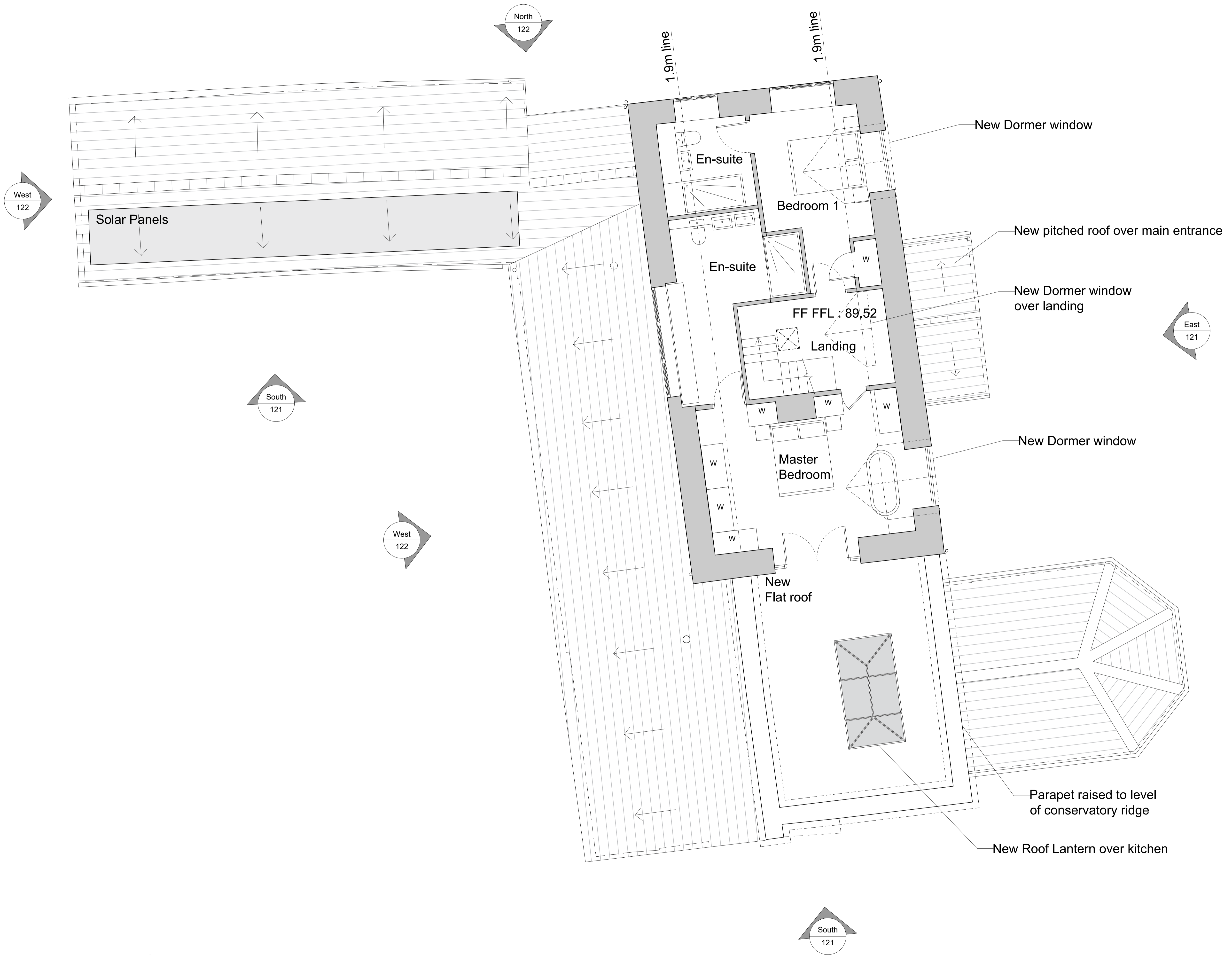
Proposed First Floor Plan 1:50 @ A1
