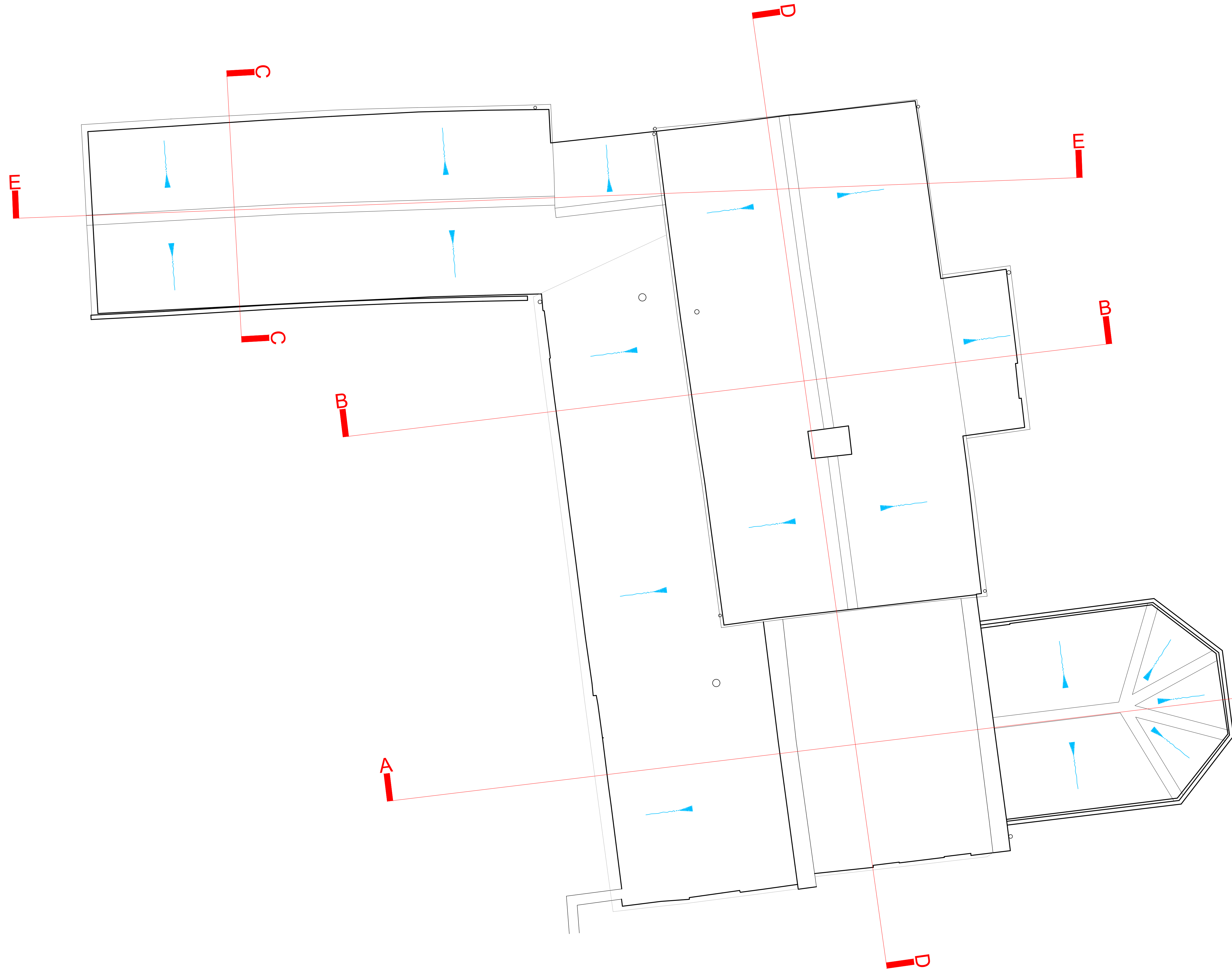
Existing Roof Plan 1:50 @ A1
