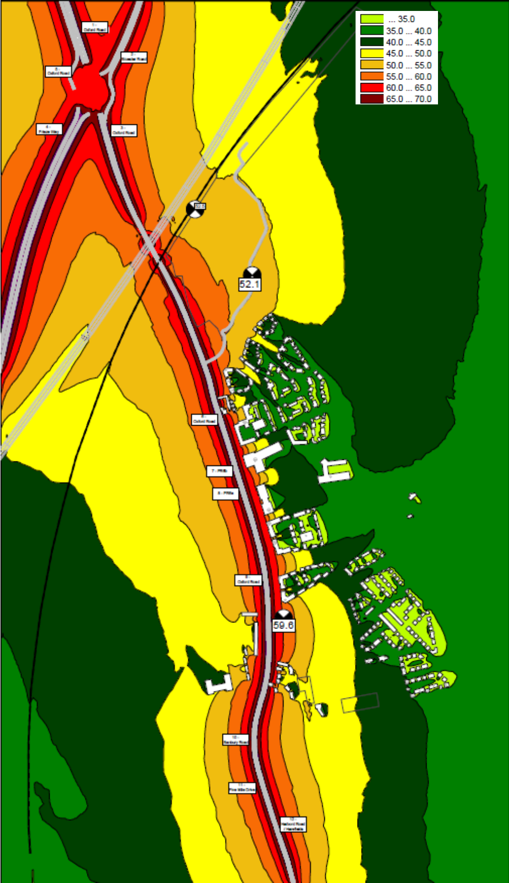
Figure 7.3 Noise levels across the Site with proposed development in place – 2023
