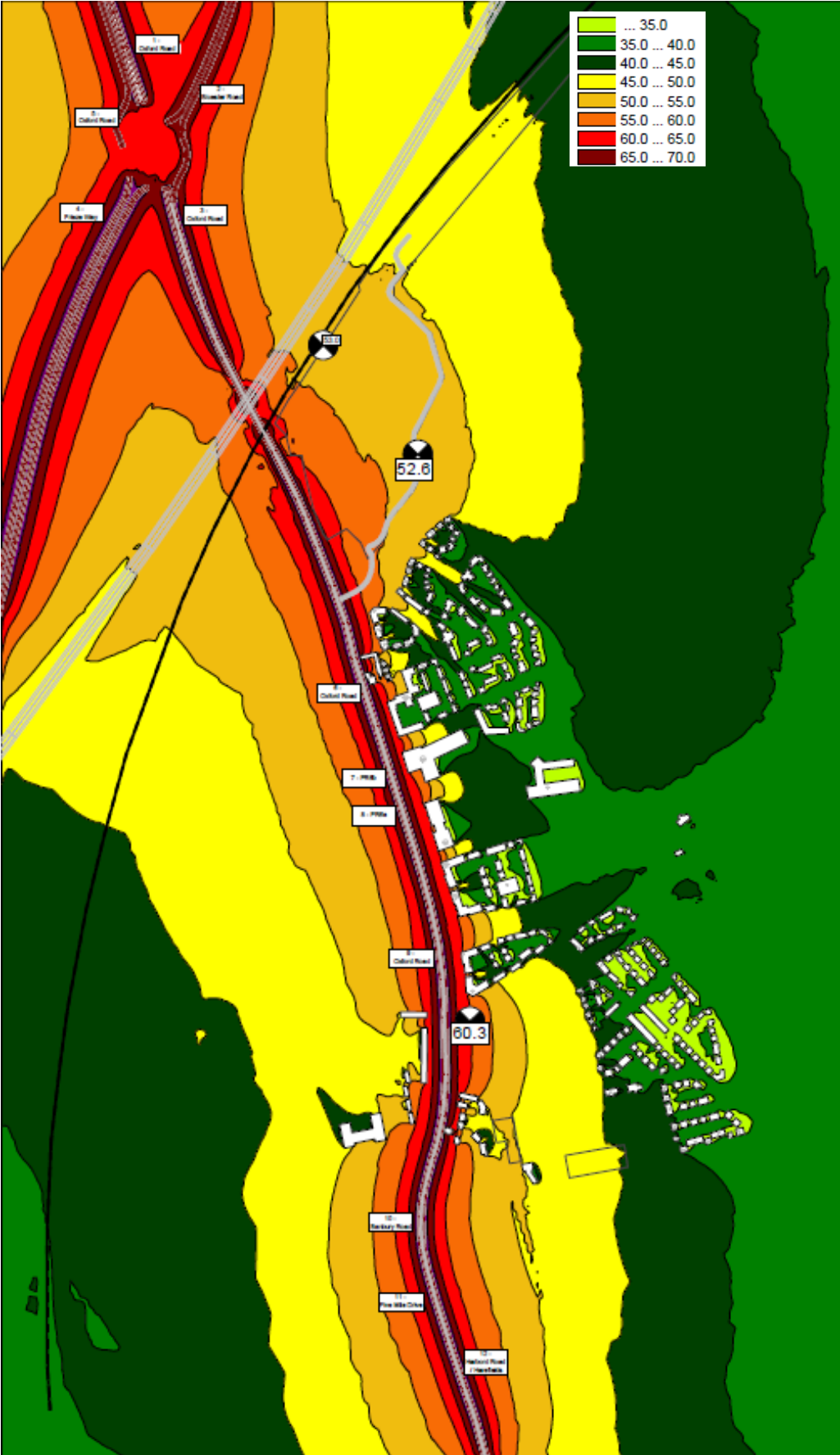
Figure 7.7 Noise levels across the Site with proposed development in place – 2031
