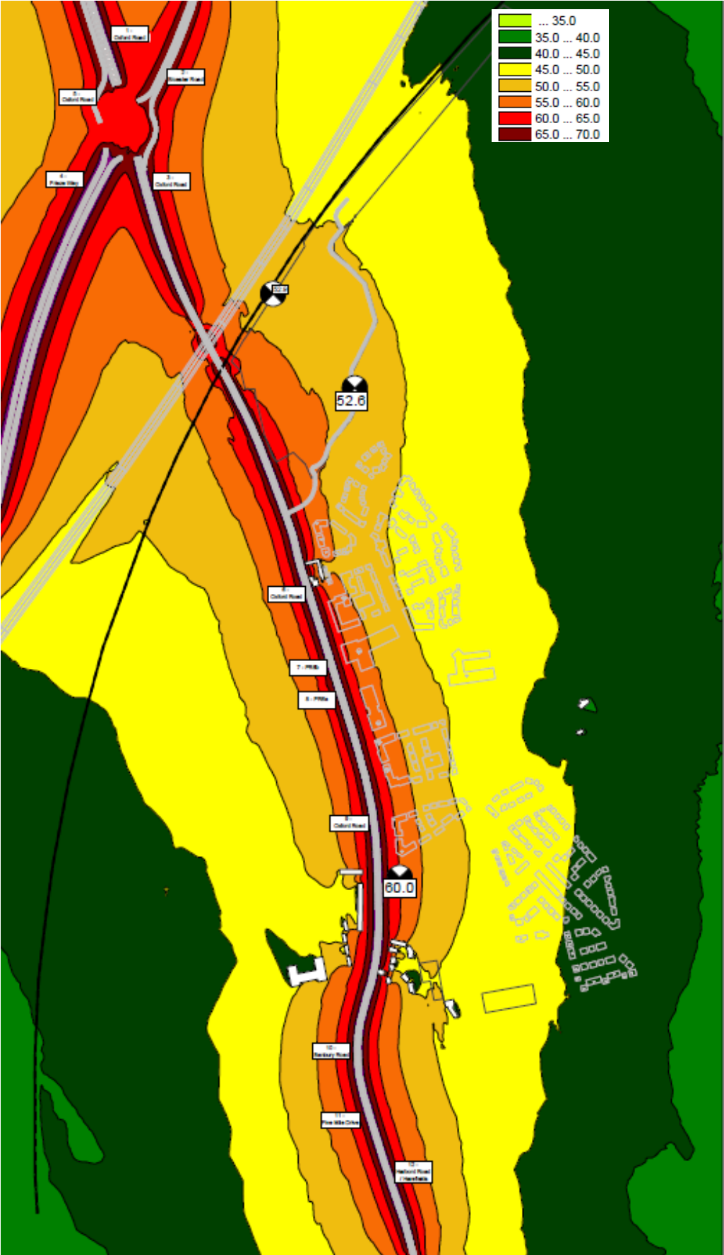
Figure 7.6 Noise levels across the Site without proposed development in place – 2031
