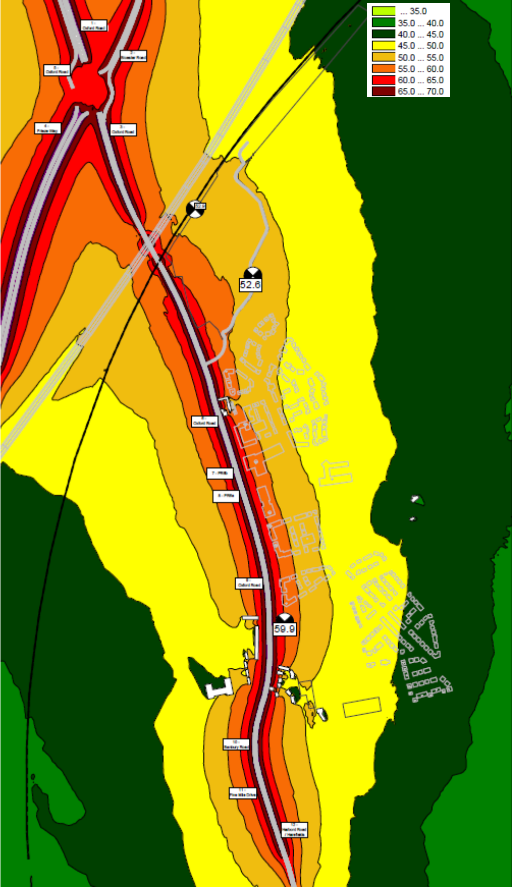
Figure 7.4 Noise levels across the Site without proposed development in place – 2025
