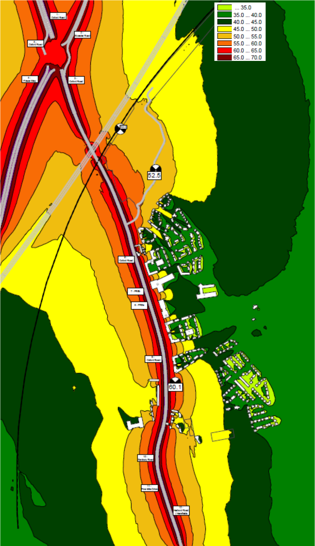
Figure 7.5 Noise levels across the Site with proposed development in place – 2025
