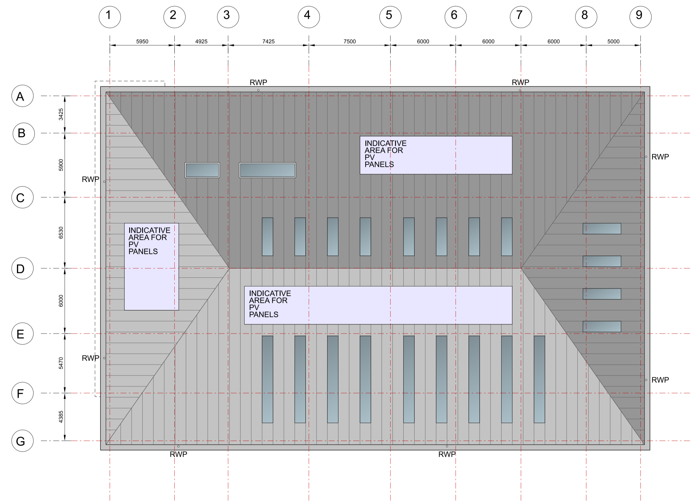
1 Unit 5 003 Roof Plan
