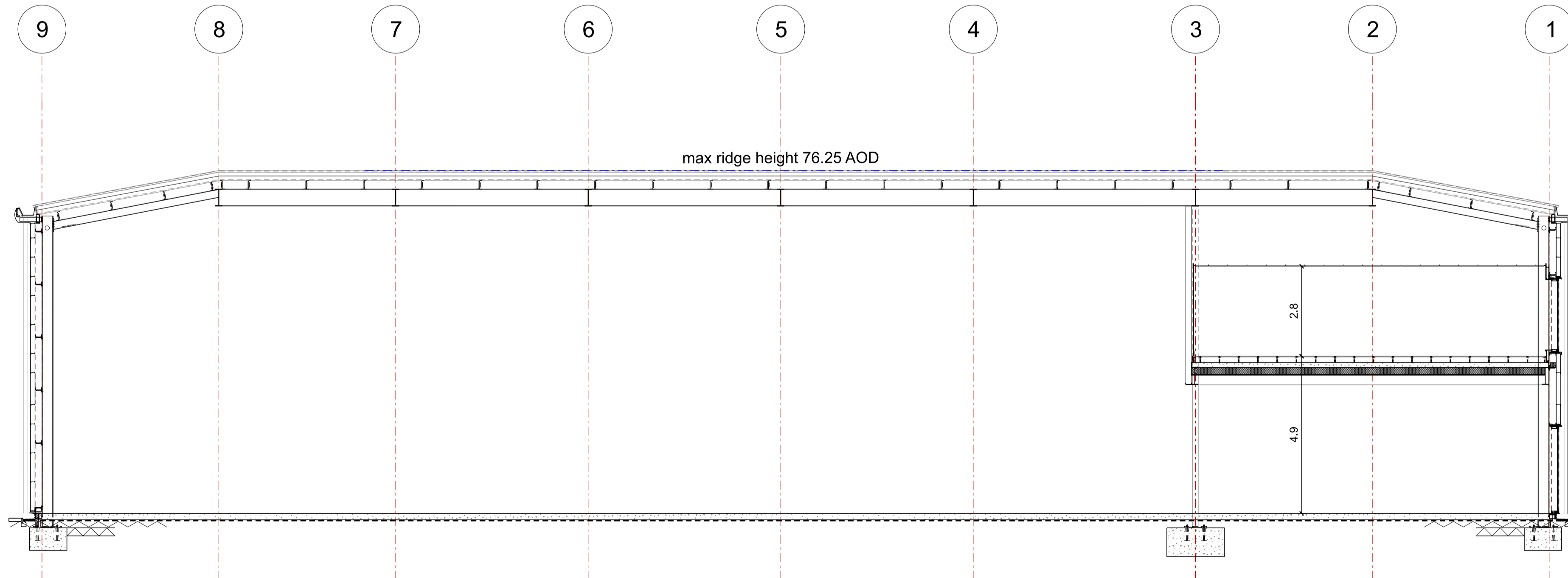
2 Unit 6 009 Long Section
