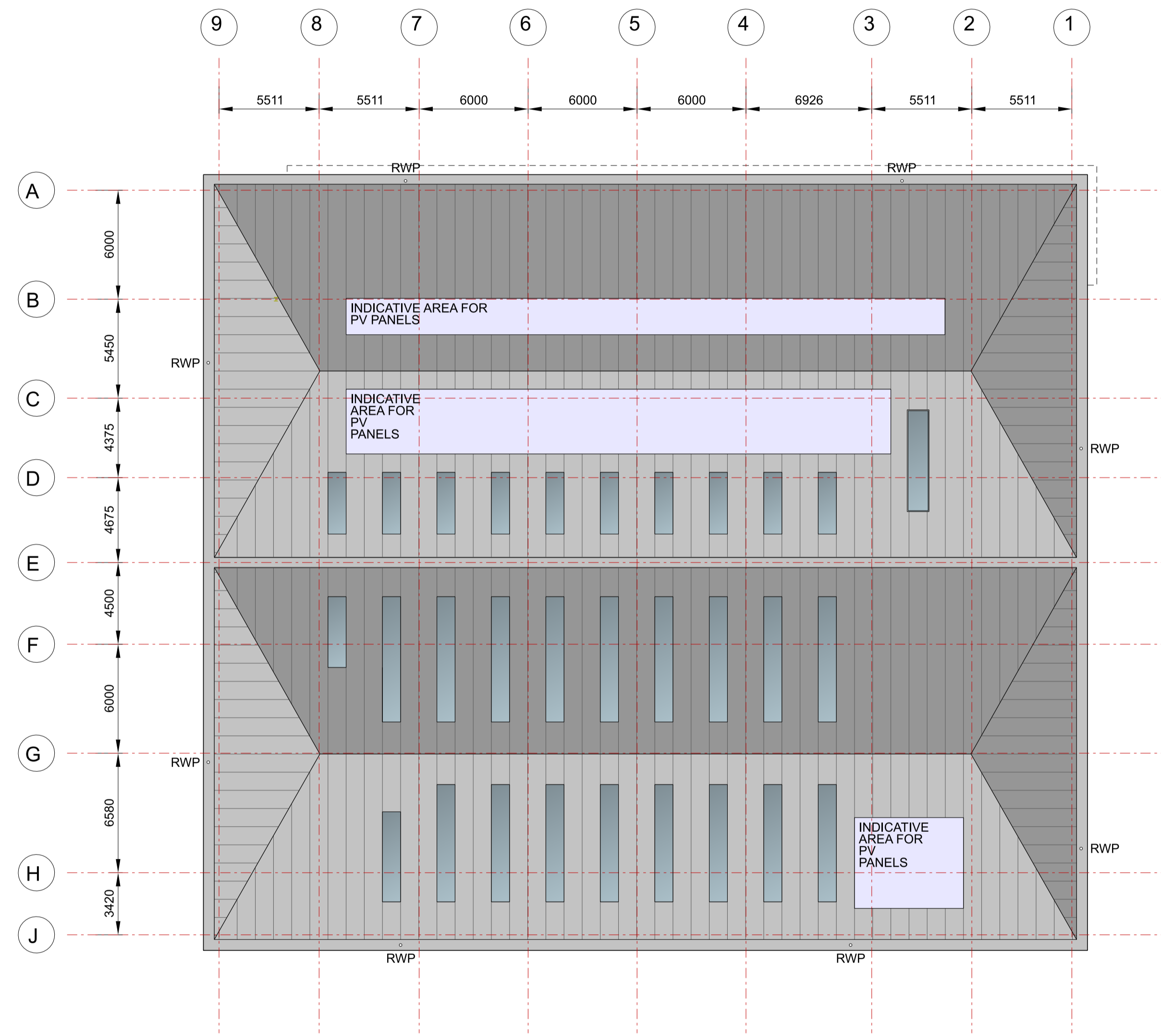
Unit 6 Roof Plan
