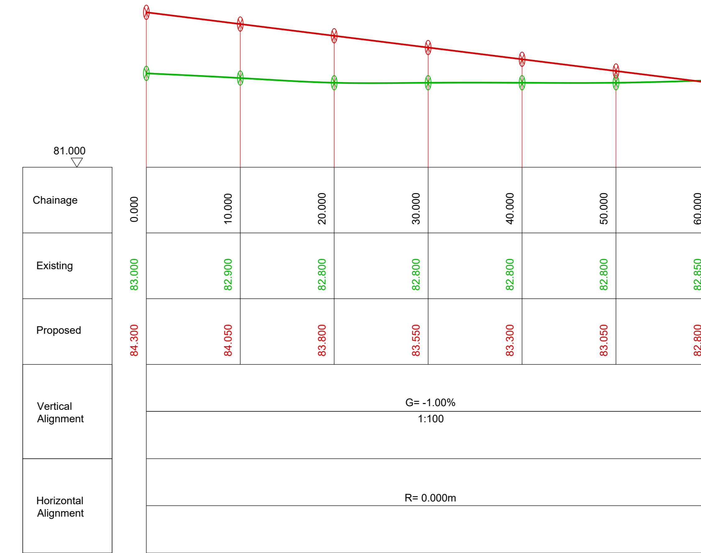
"Howes Lane link footway" Longitudinal Section 1:250(H) 1:50(V)
