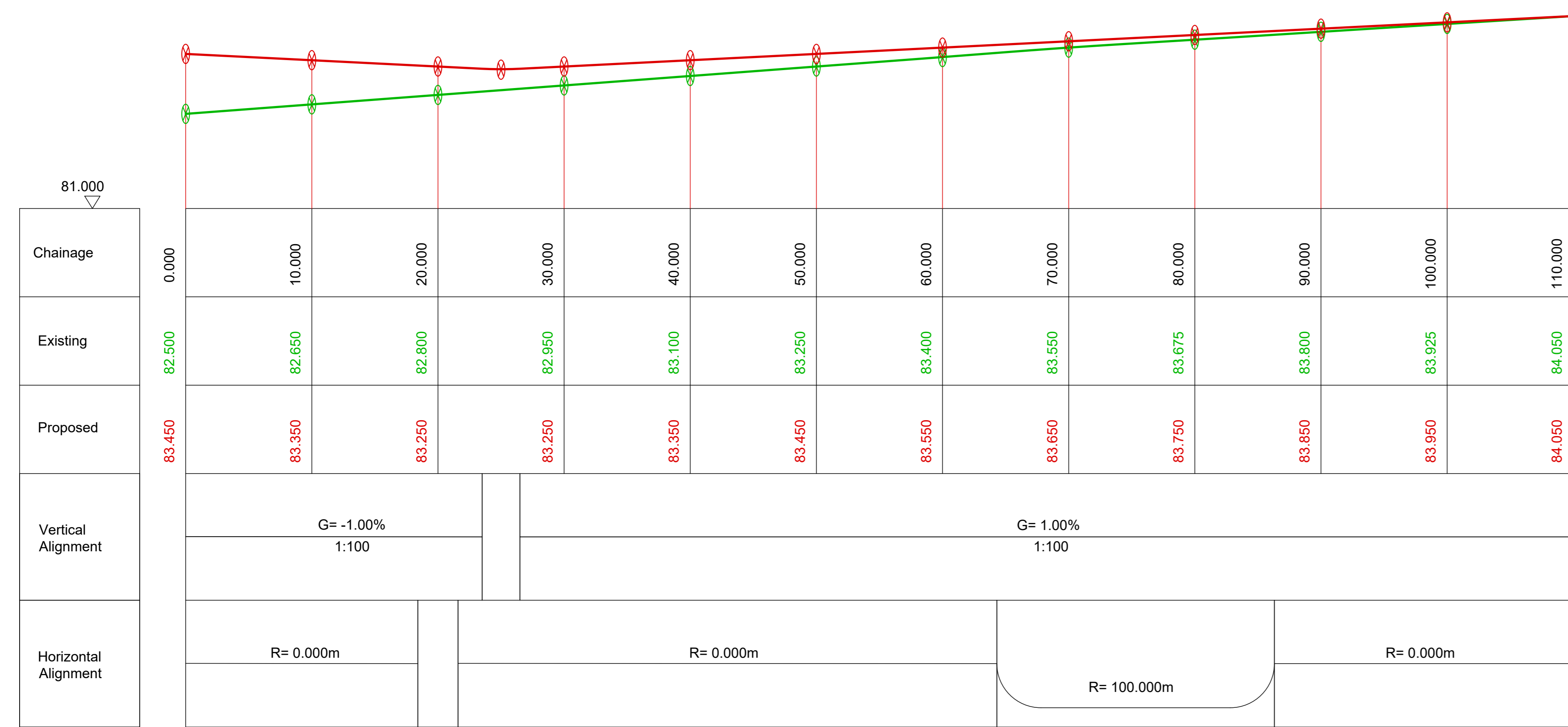
"Empire Road Extension" Chainage 0m to 110m Longitudinal Section 1:250(H) 1:50(V)
