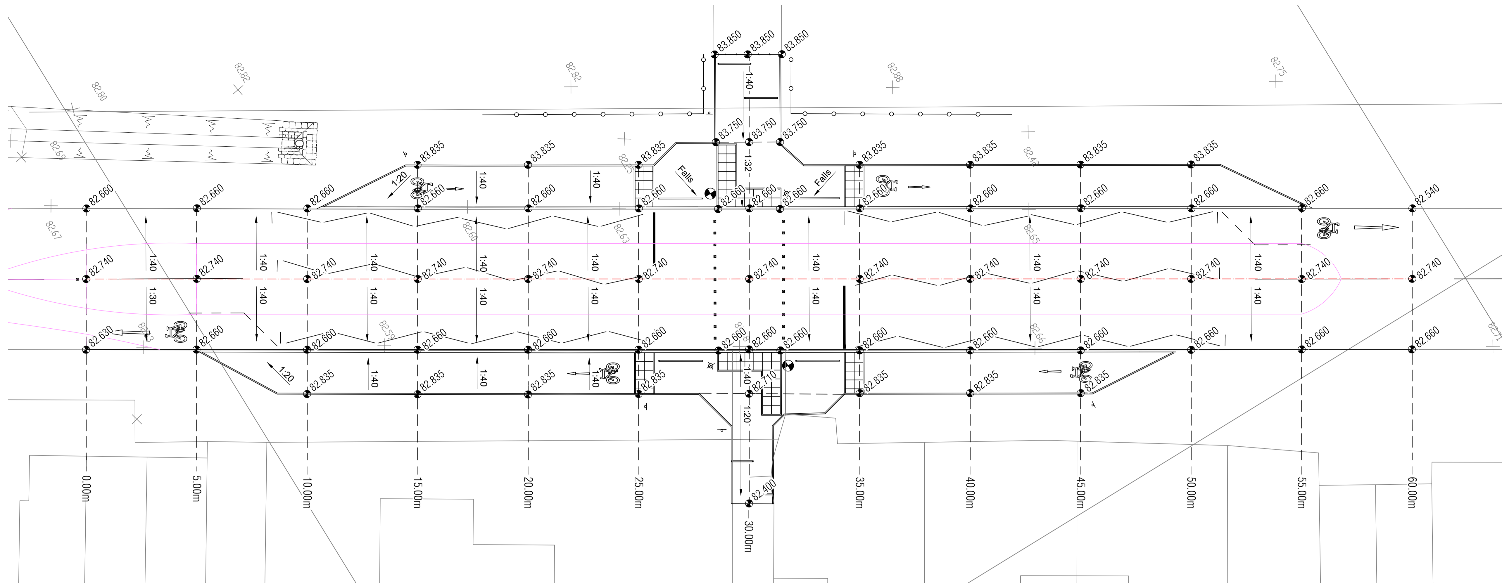
Levels & Contours Plan 1:100
