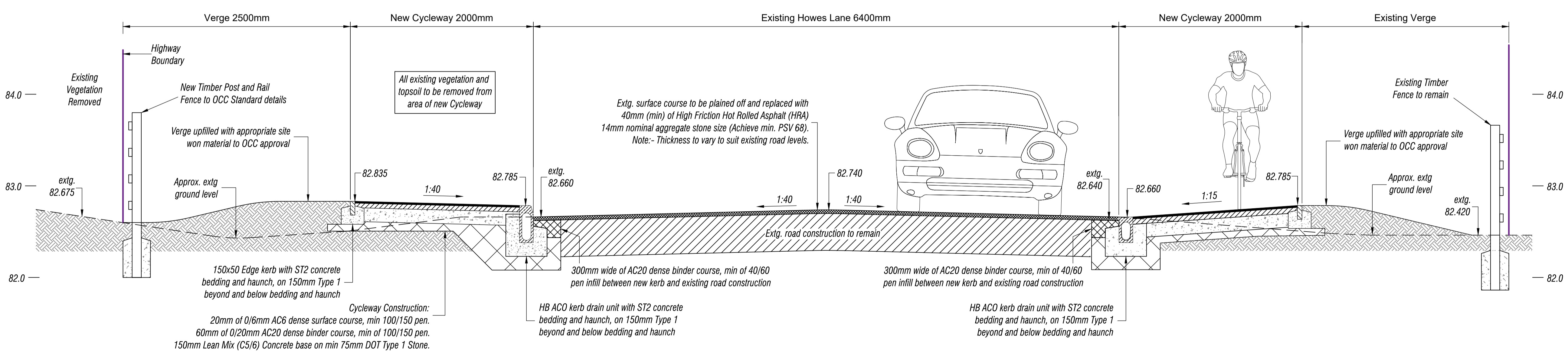
Section C-C Chainage 45m (1:25)
