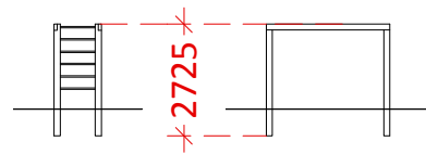
Front Elevation Side Elevation MONKEY BARS SEE 1. ON DWG NO. 1-04
