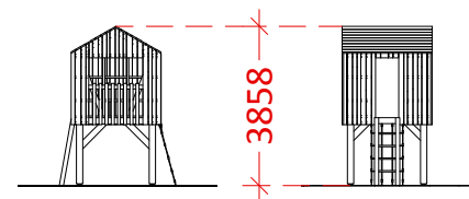
Front Elevation Side Elevation WILDLIFE OBSERVATION AND STUDY HUT SEE 19. ON DWG NO. 1-04
