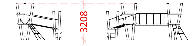
Front Elevation CLIMBING FRAME SEE 20. ON DWG NO. 1-04
