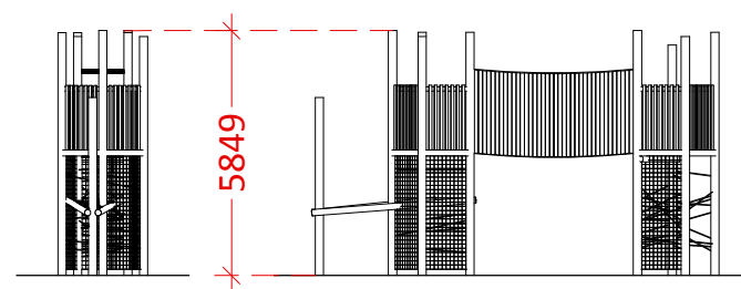
Front Elevation CLIMBING FRAME SEE 10. ON DWG NO. 1-04
