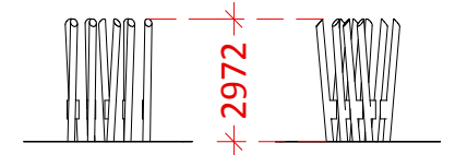
Front Elevation STEPPING POLES TRAIL SEE 7. ON DWG NO. 1-04
