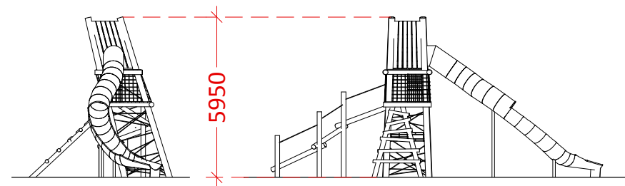
Front Elevation CLIMBING FRAME SEE 2. ON DWG NO. 1-04
