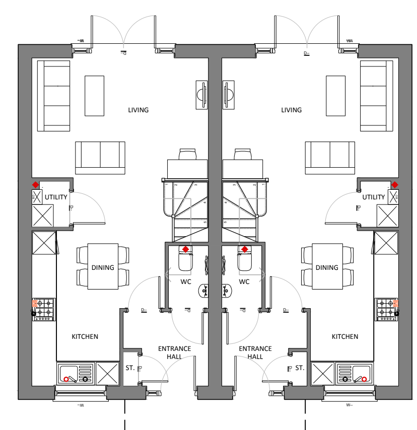
Ground Floor Plan M4(2) Compliant Housetype
