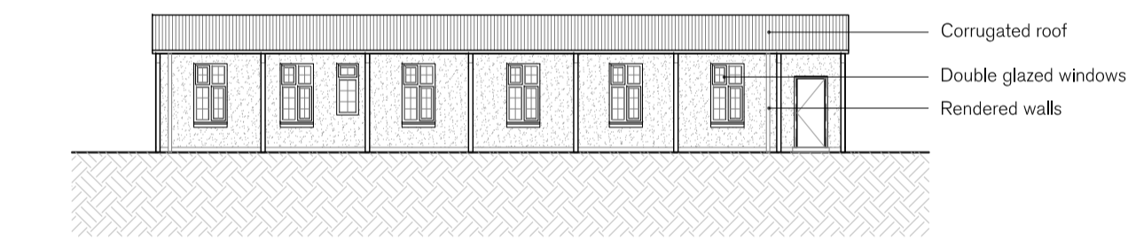
Elevation C 1:200
