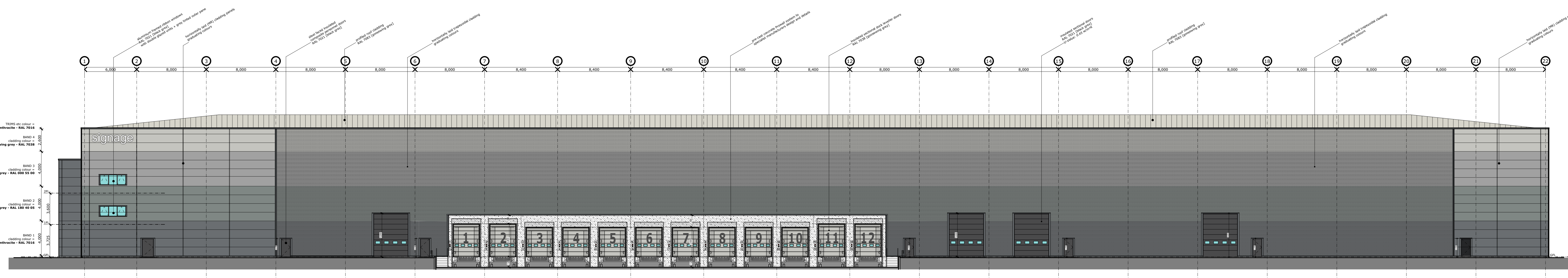
right side / west elevation
