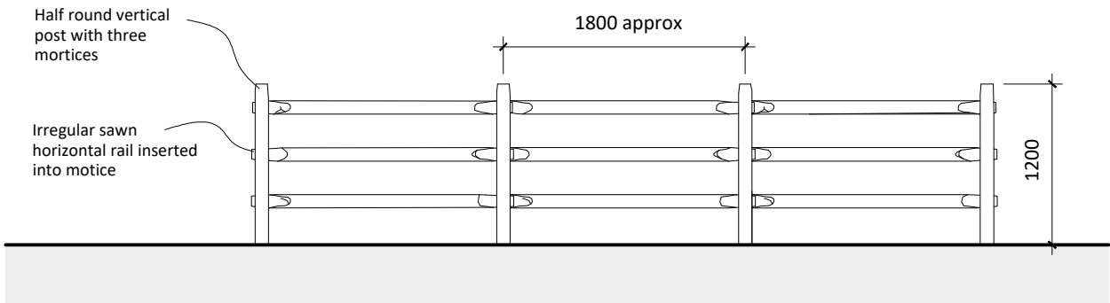
ELEVATION - Proposed Heavy Mortice Fence 1:50
