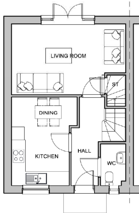
GROUND FLOOR PLAN GIA = 79sqm
