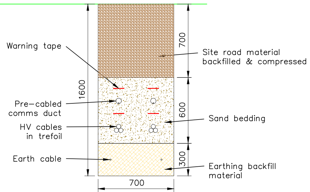
Typical HV AC trench roadway/crossing points
