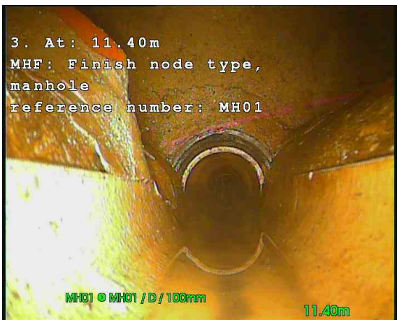
221114_1653A-Survey.jpg, 00:00:57, 11.40 m Finish node type, manhole, reference number: MH01
