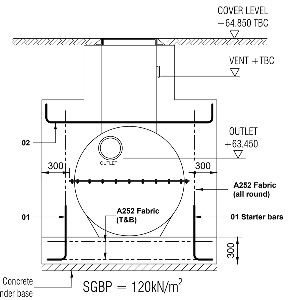
SECTION B-B 1:25
