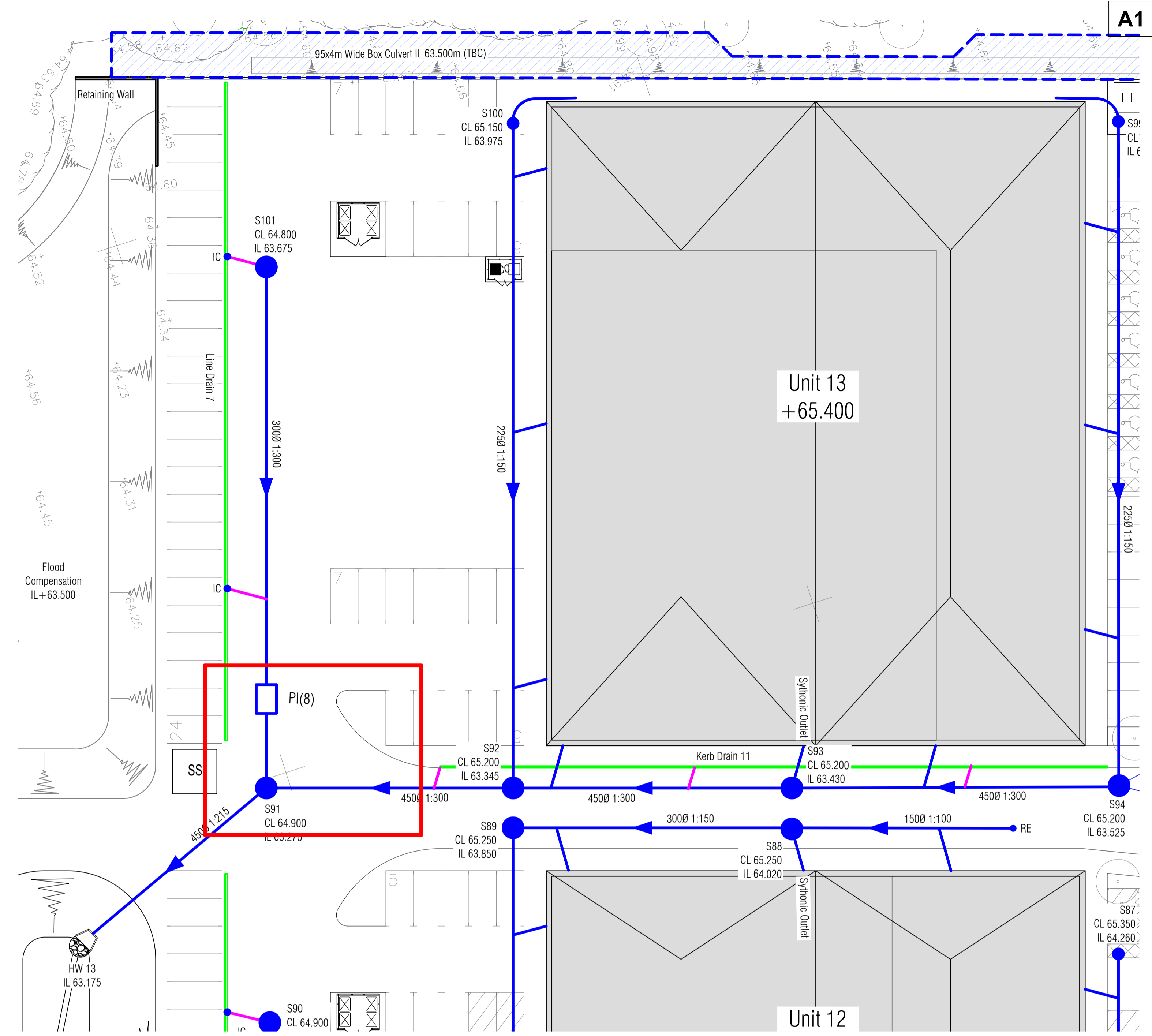
Unit 13 Drainage Key Plan 1:250
