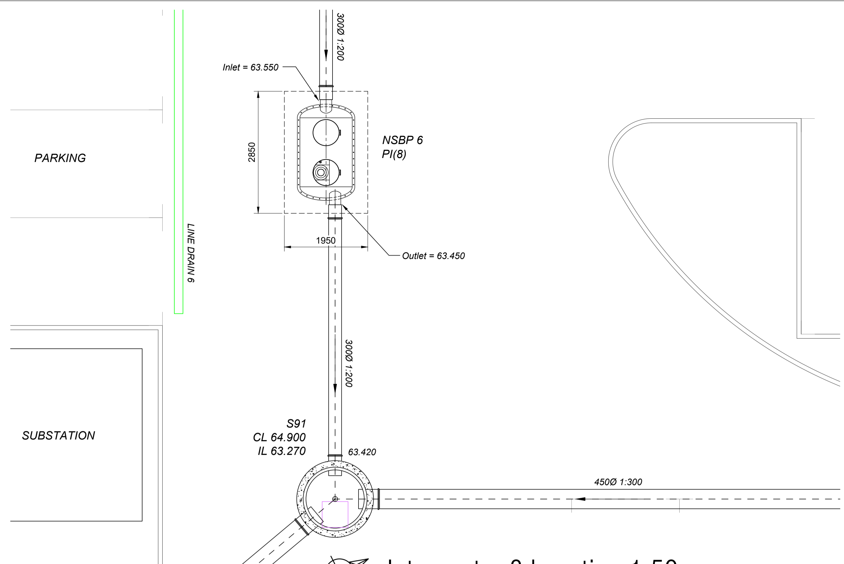
Interceptor 8 Location 1:50
