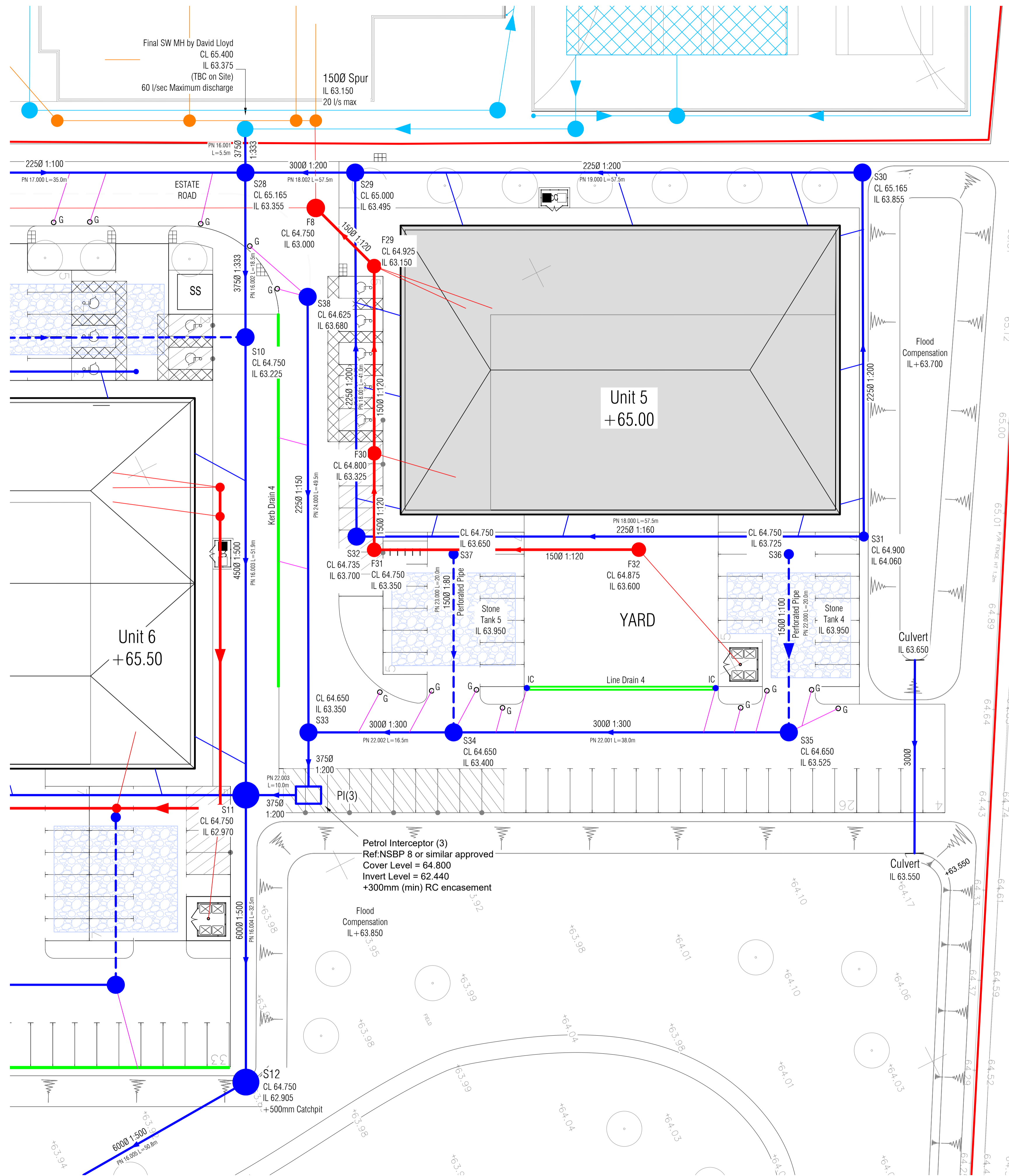
Unit 5 Drainage Layout 1:250
