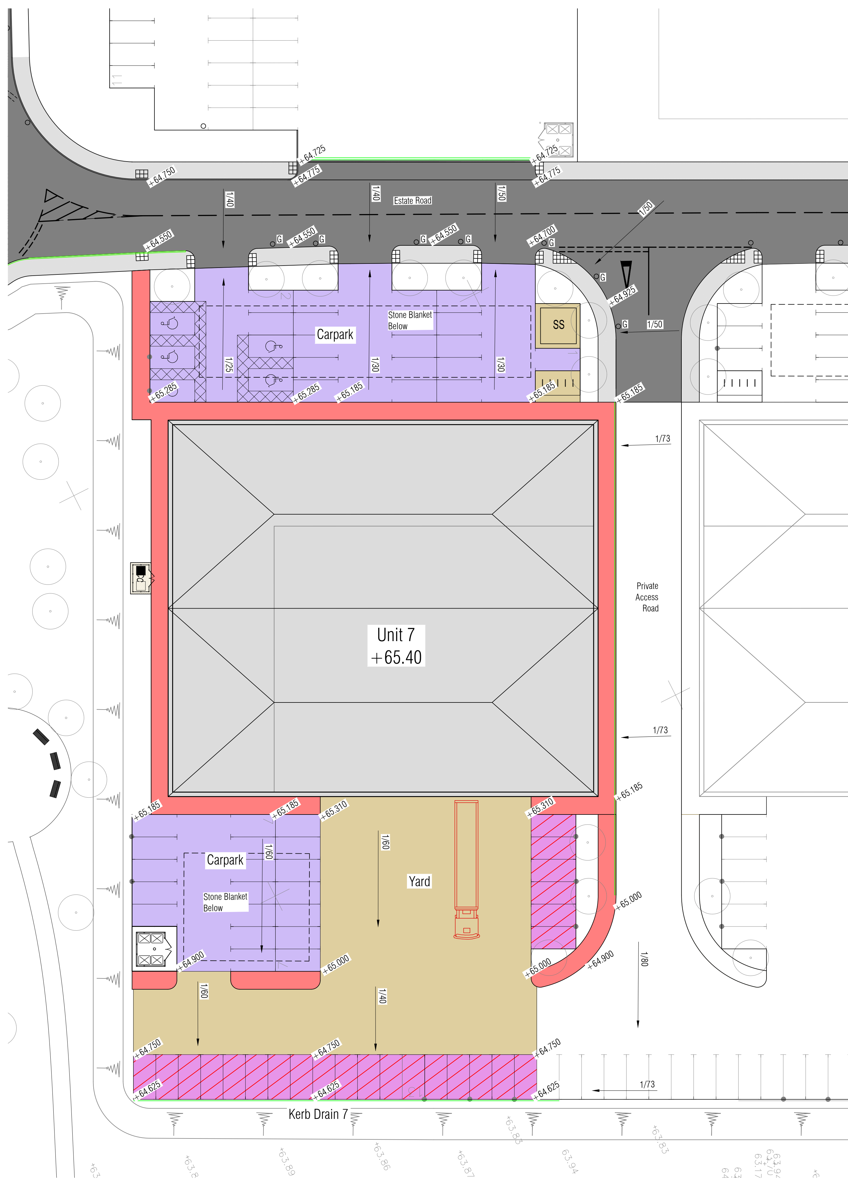
Unit 7 External Works Layout 1:250
