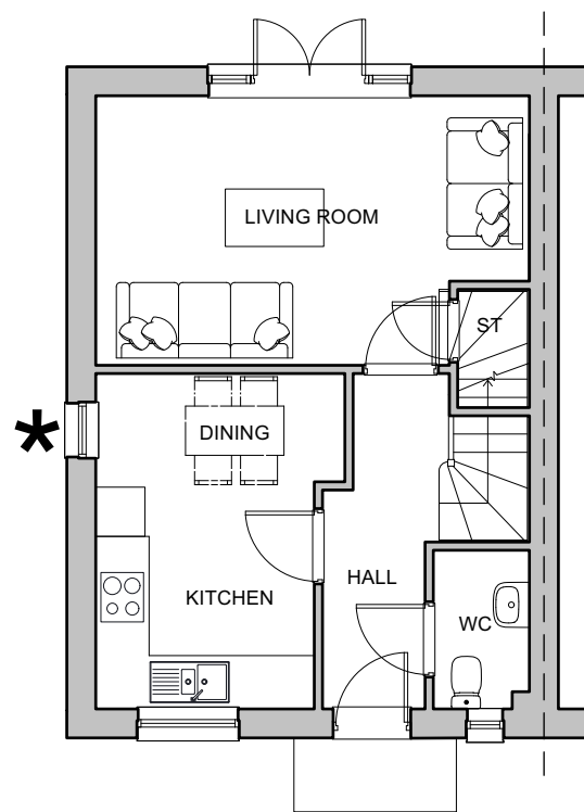
GROUND FLOOR PLAN GIA = 79sqm
