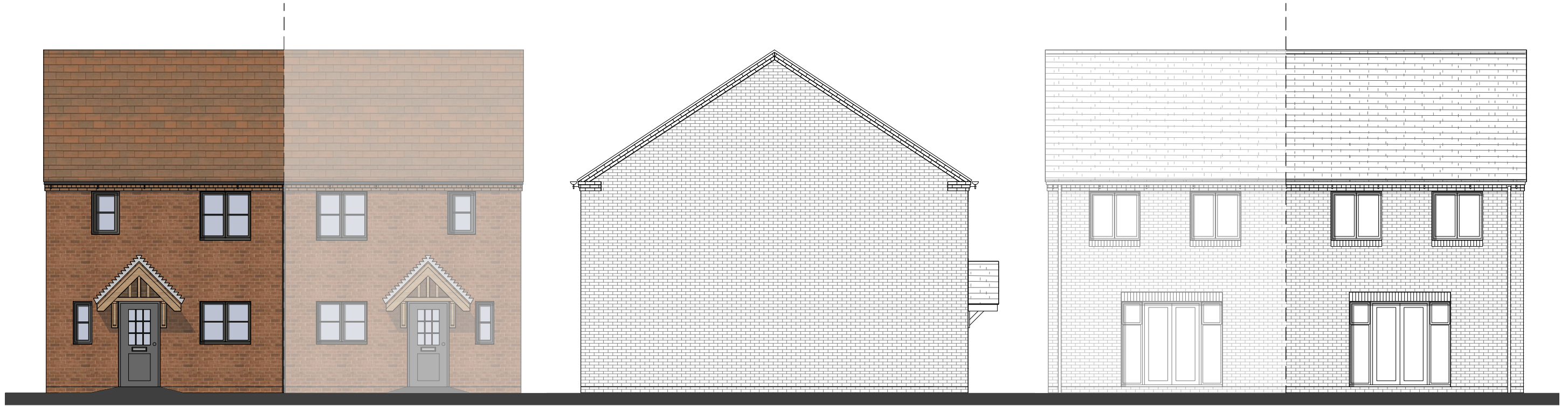
FRONT ELEVATION
