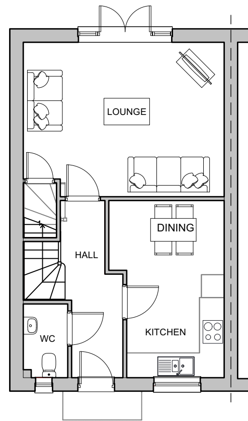
GROUND FLOOR PLAN GIA = 93sqm
