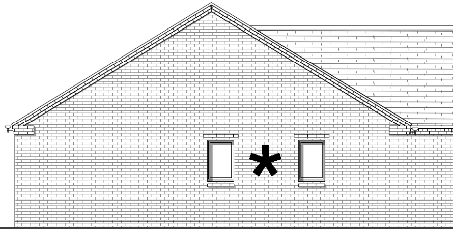
SIDE ELEVATION
