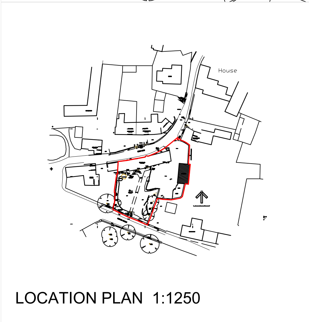
BLOCK PLAN 1:500
