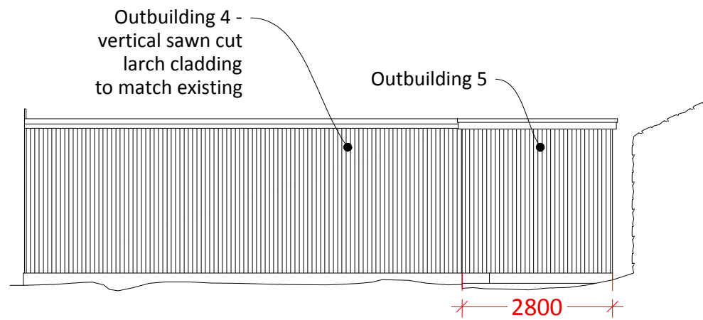
East Elevation 1:100
