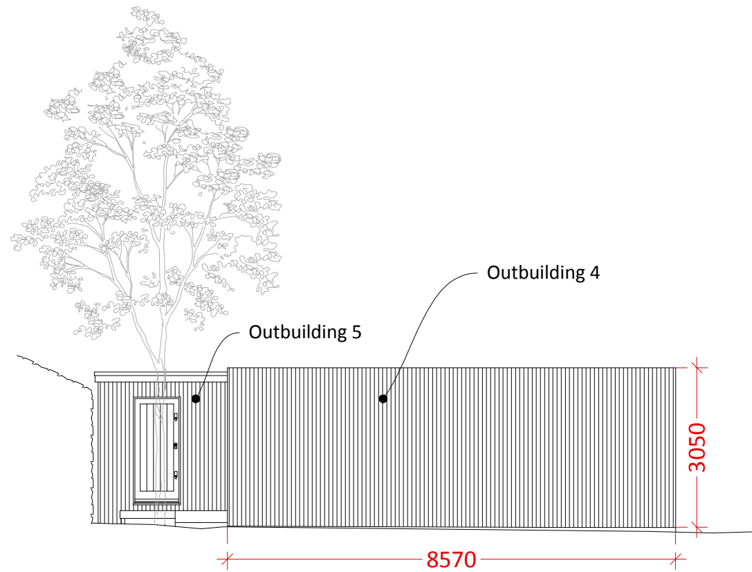
West Elevation 1:100
