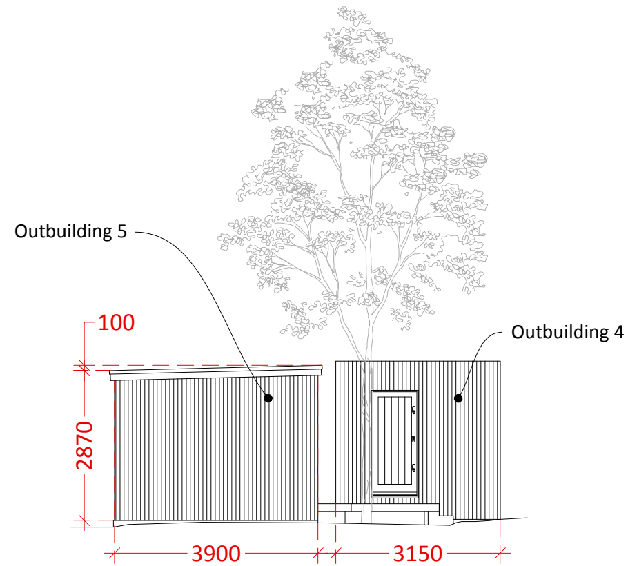
North Elevation 1:100
