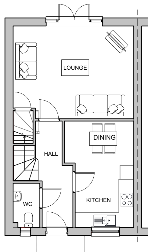
GROUND FLOOR PLAN GIA = 93sqm
