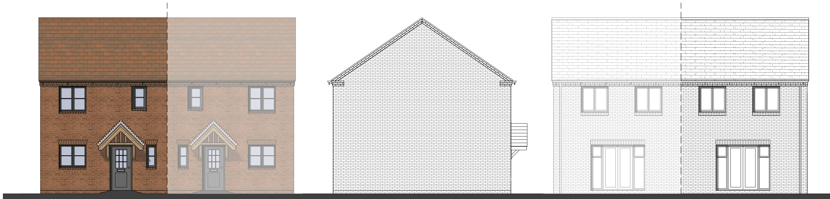
FRONT ELEVATION STANTON
