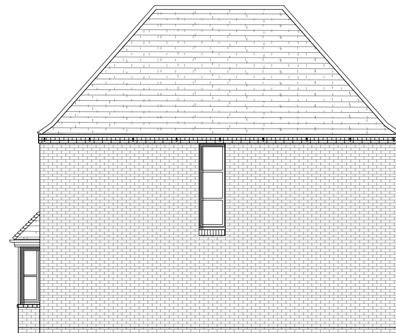
REAR ELEVATION
