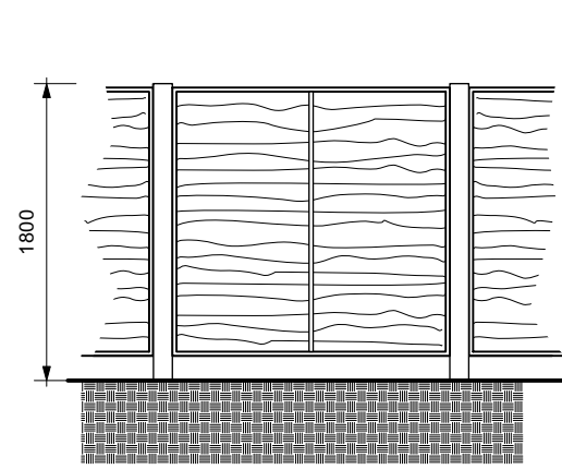
1.8m High Panel Fence
