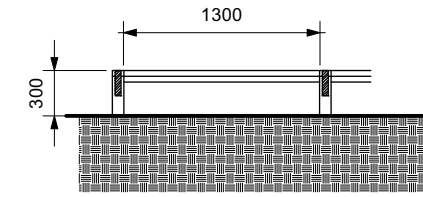
0.3m High timber knee rail
