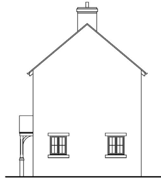
SIDE ELEVATION
