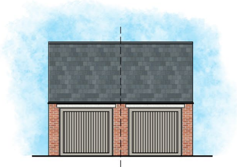
PLOT 28 PLOT 29 FRONT ELEVATION
