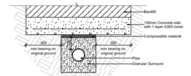
Concrete Protection for Pipes Laid at Shallow Depths Cover < 600mm
