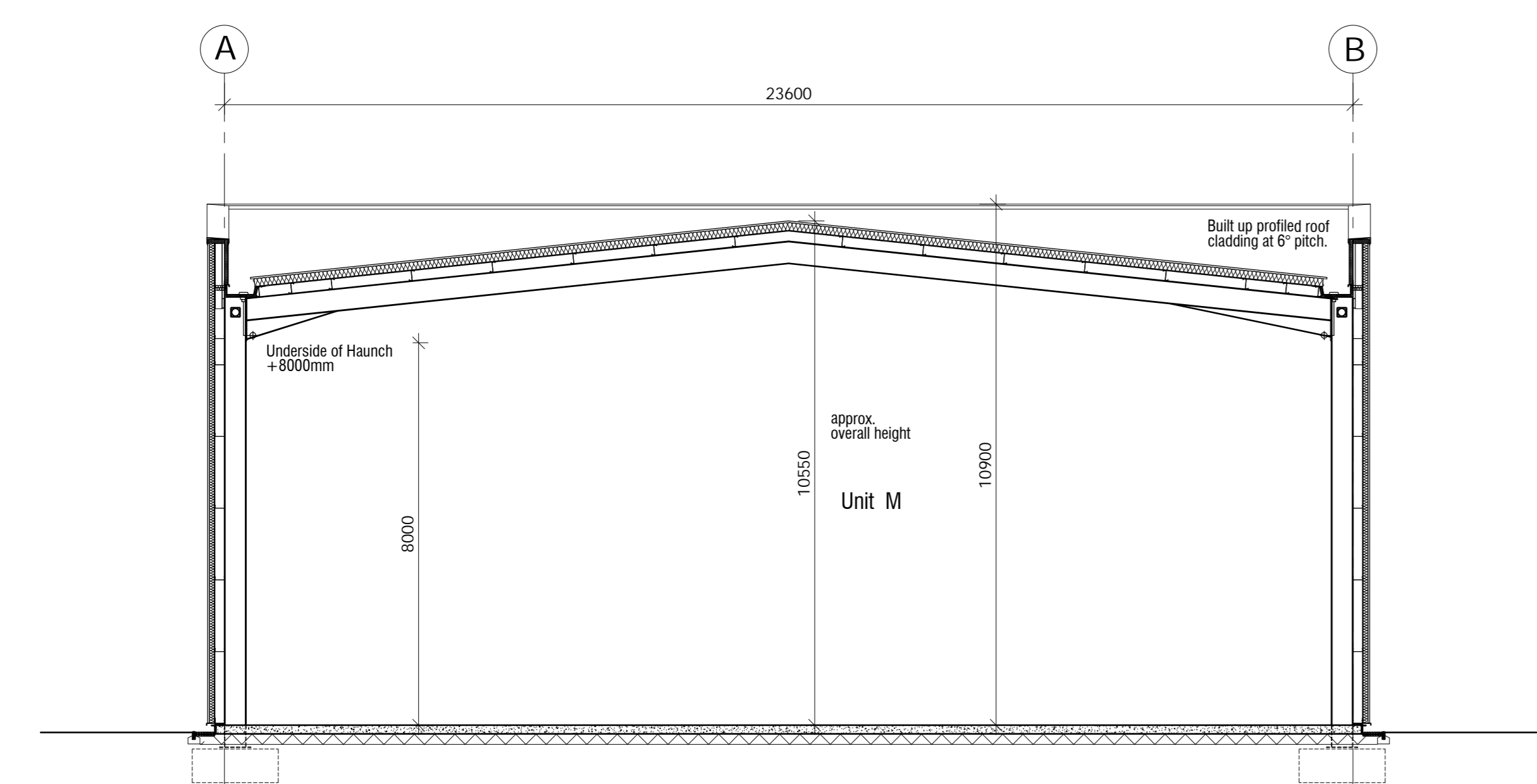
Section B - B
