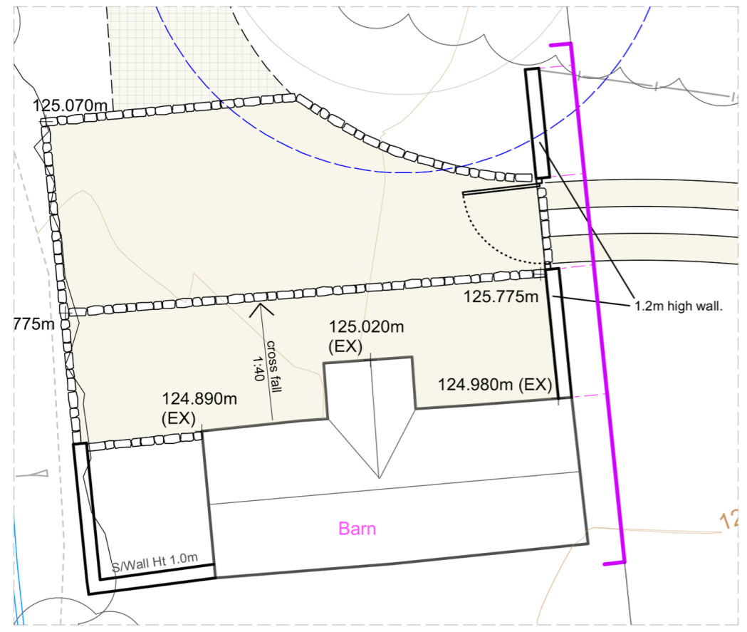
BARN & ENTRANCE LAYOUT: ELEVATION AA
